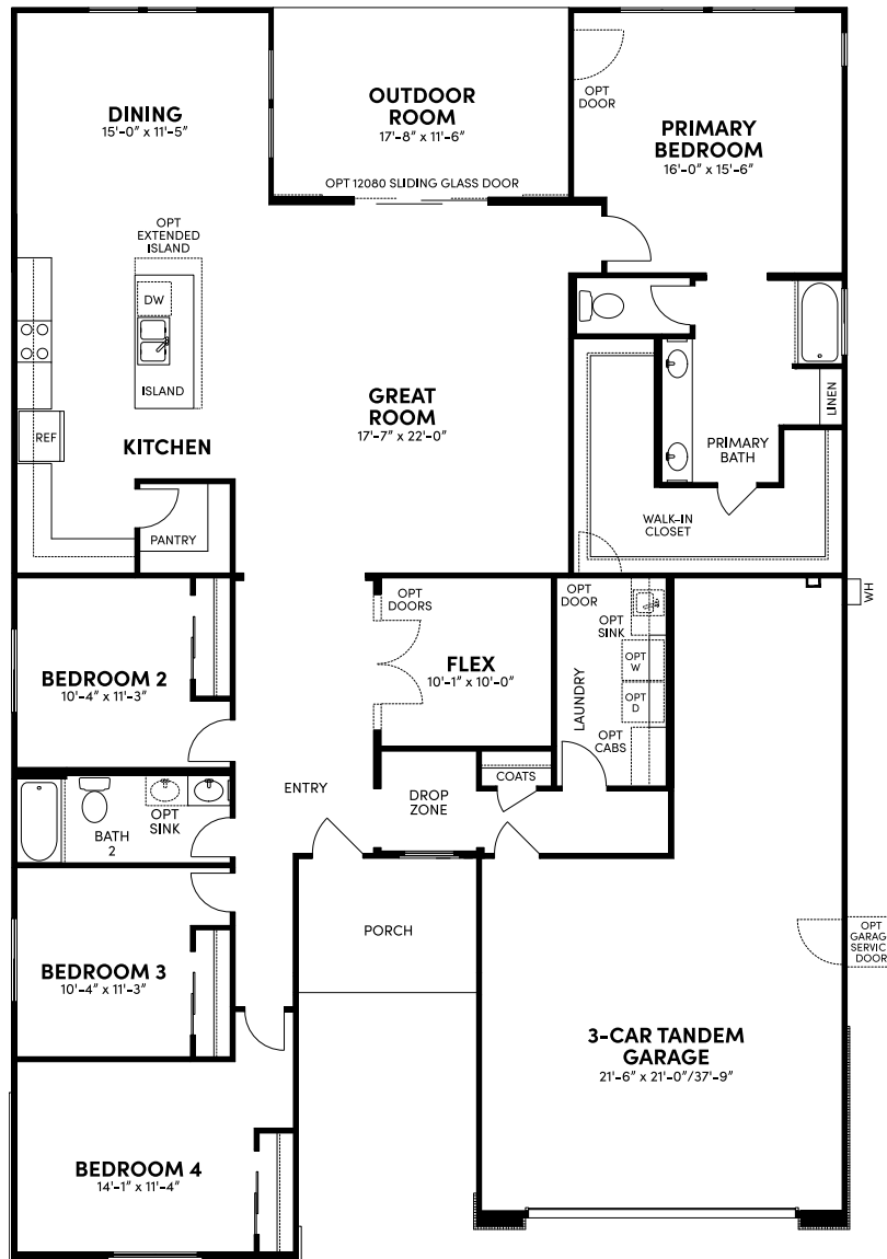
ONE-STORY – INCLUDED PLAN
