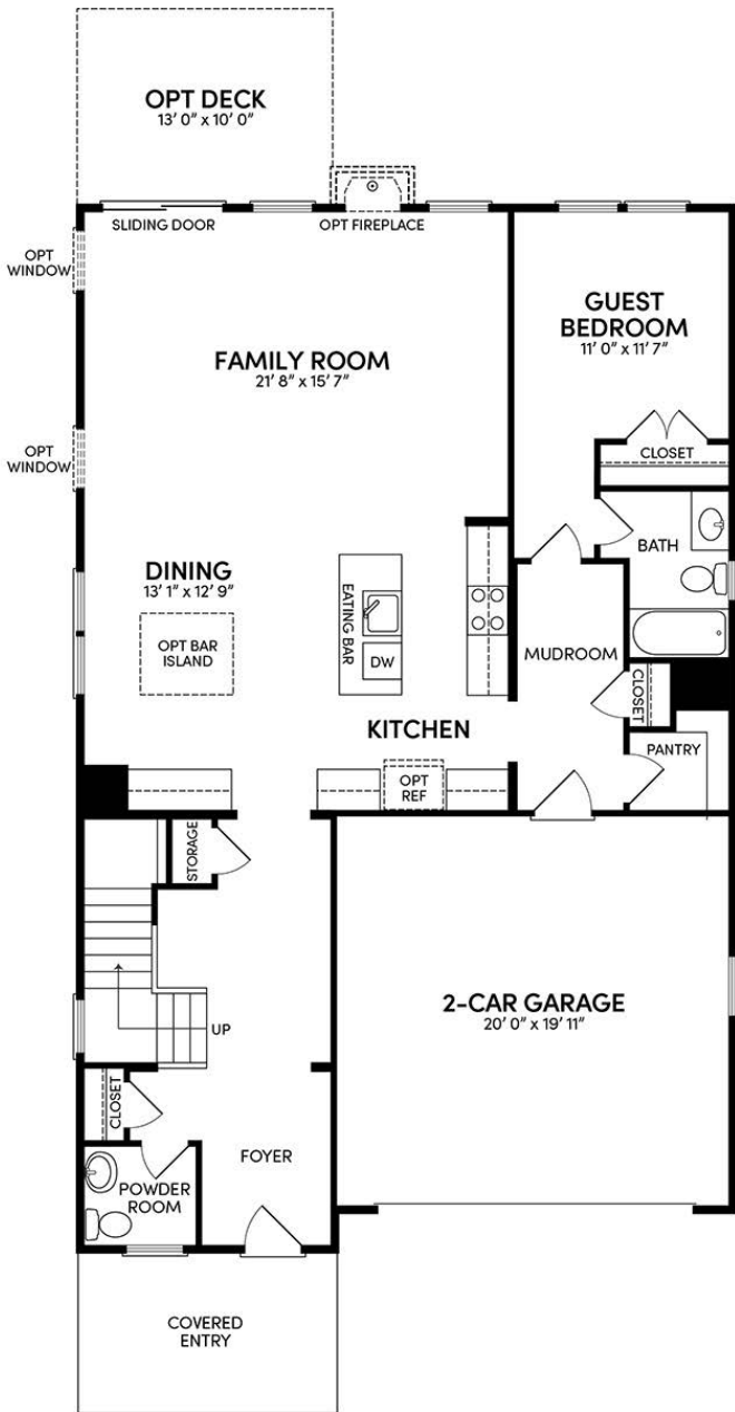
Floor 1
