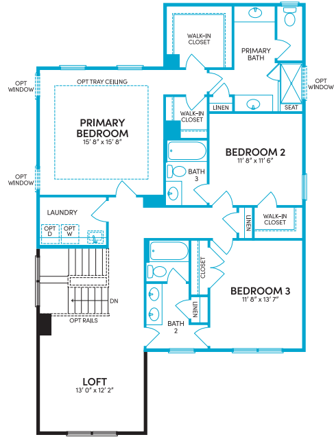
Floor 2 with Optional Extension
