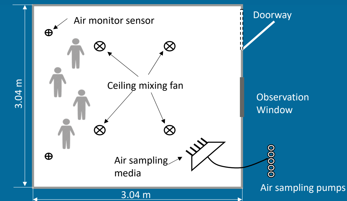
Figure 1. Environment Chamber
