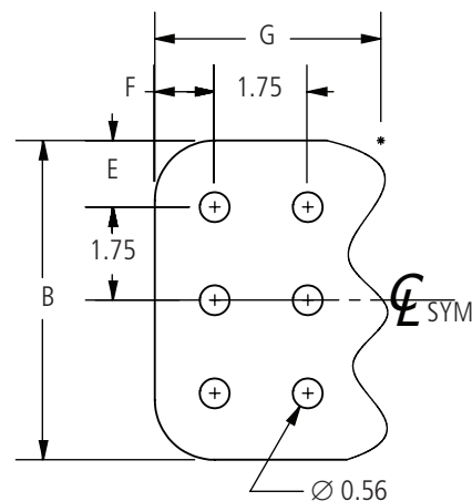
Pad Detail 2
