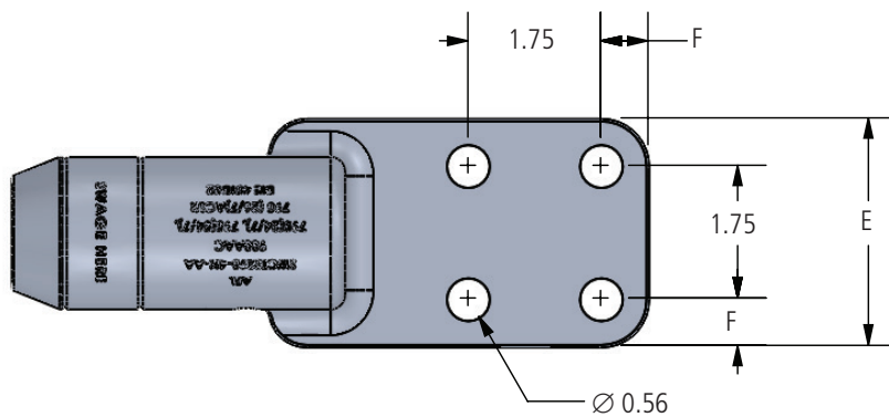
Pad Detail 2
