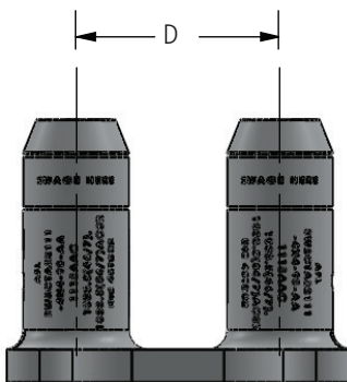
Pad Detail 1
