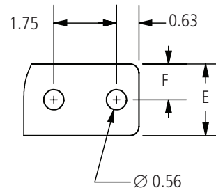
Pad Detail 1
