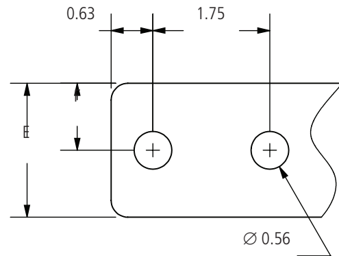
Pad Detail 1
