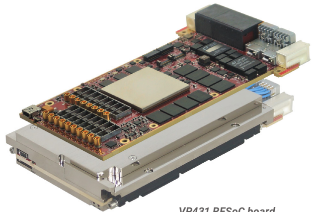
VP431 RFSoc board
