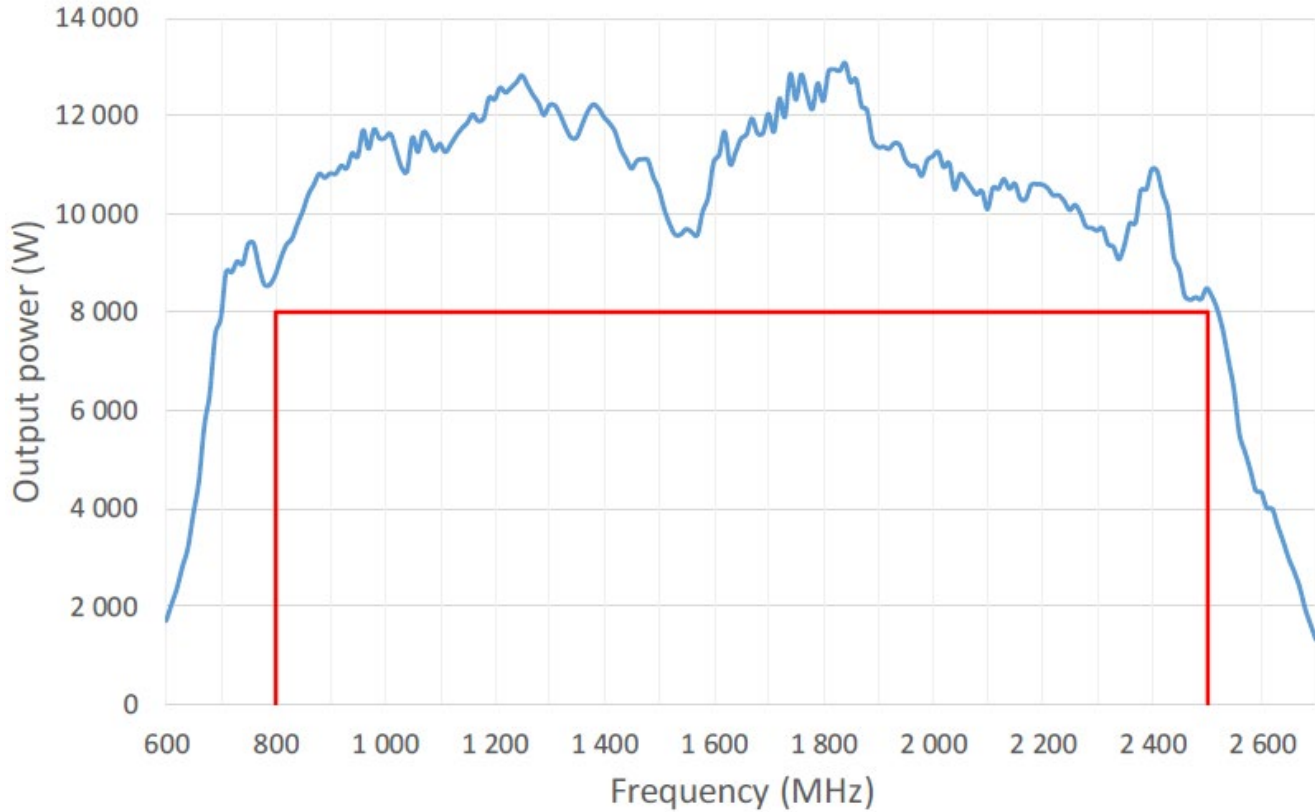
Typical Output Power ( P_{sat} @ 0 dBm input)
