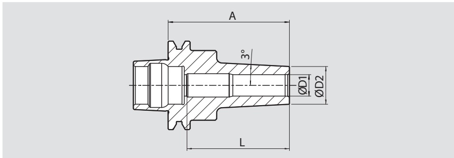
HSK 25 Mini-Shrink HSK tool holder with special Kern design similar to HSK-E25
