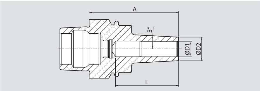
HSK 40 Mini-Shrink HSK tool holder with special Kern design similar to HSK-E40
