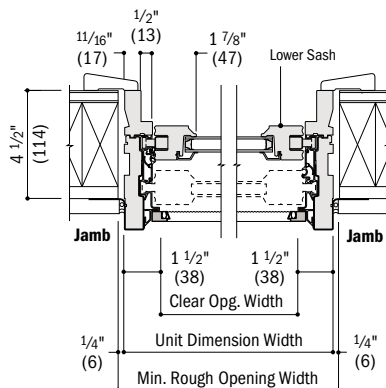
Horizontal Section
