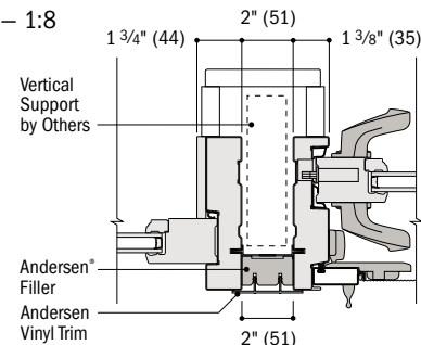
Horizontal Section
