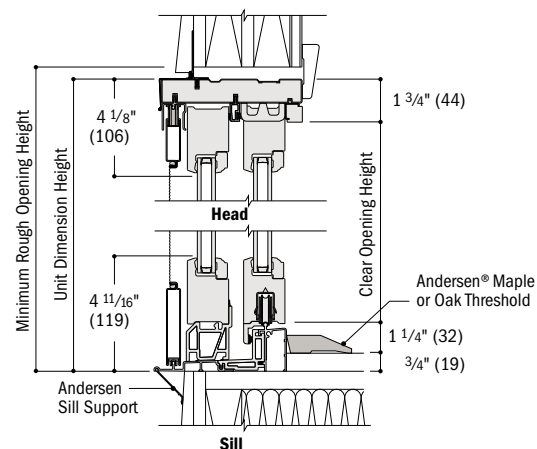
Vertical Section
