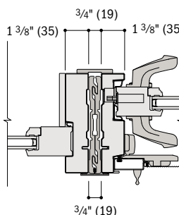
Horizontal Section
