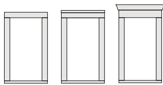
Flat casing on three sides with sill nose with optional decorative drip cap or cornice.
