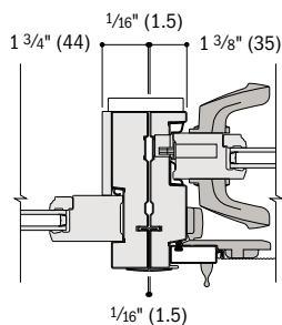
Horizontal Section
