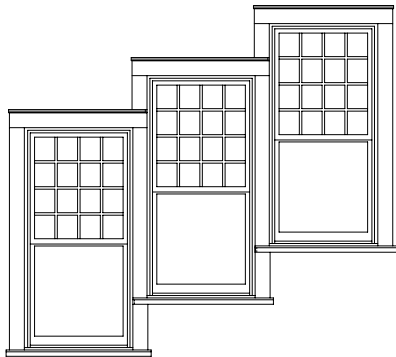
Three-wide double-hung stepped window grouping with wide mullions
