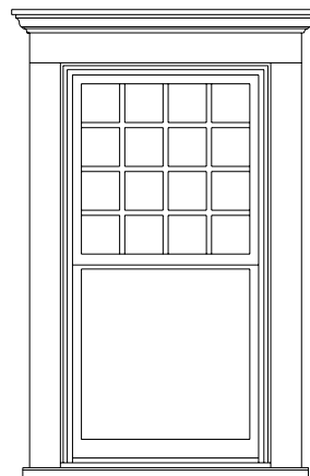
Flat trim for jamb and head with extended sill nose and 3 ⅝" cornice
