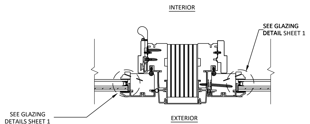
D 8 HORIZONTAL SECTION INSULATED GLASS 2" X 3-1/2" MULLION
