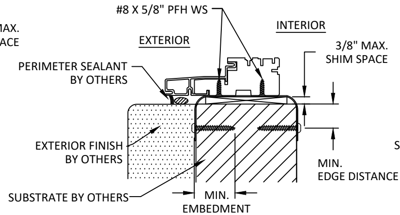
B 9 ANCHOR DETAIL STRAP ANCHOR
