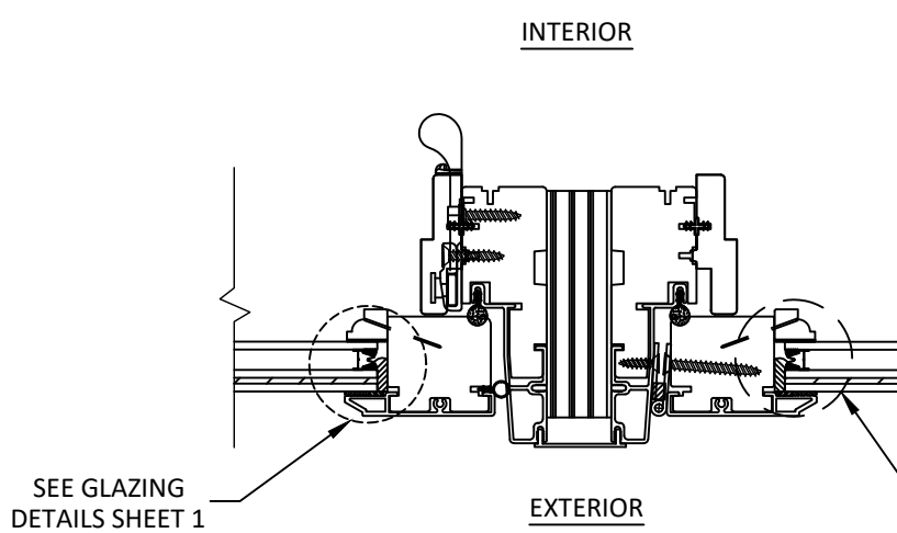
C 8 HORIZONTAL SECTION INSULATED GLASS 1" X 3-1/2" MULLION
