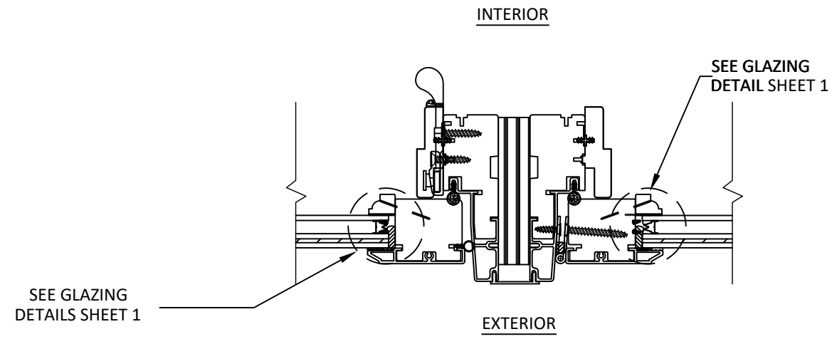
B 8 HORIZONTAL SECTION INSULATED GLASS 3/4" X 3-1/2" MULLION
