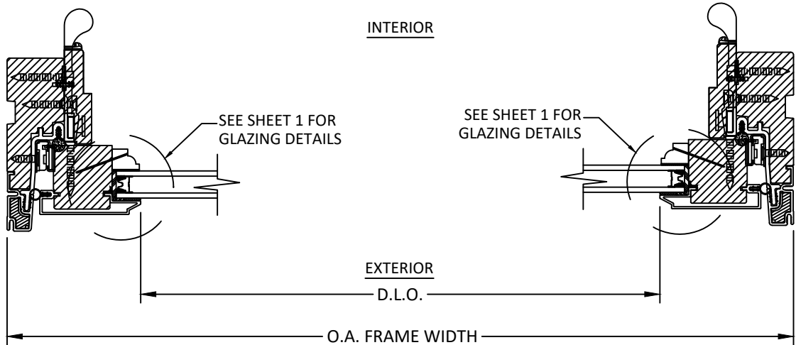
A 8 HORIZONTAL SECTION INSULATED GLASS
