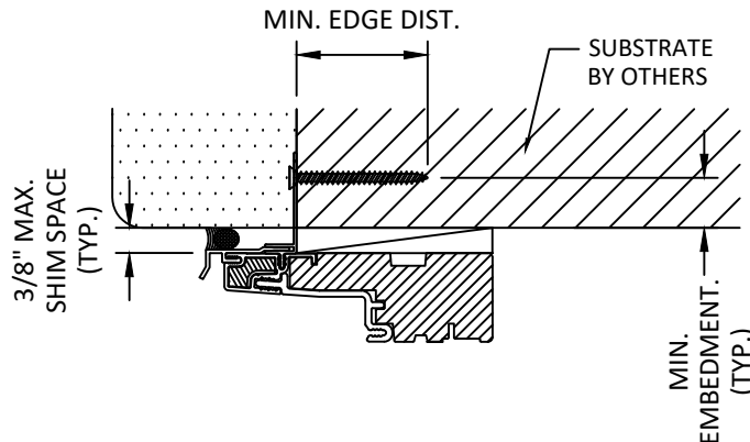
E 10 ANCHOR DETAIL VINYL NAIL FIN - HEAD ONLY
