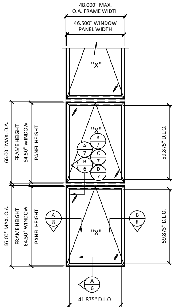
ELEVATION MULLED UNITS (WITH 2" MULLION) VERTICAL CONFIGURATION
