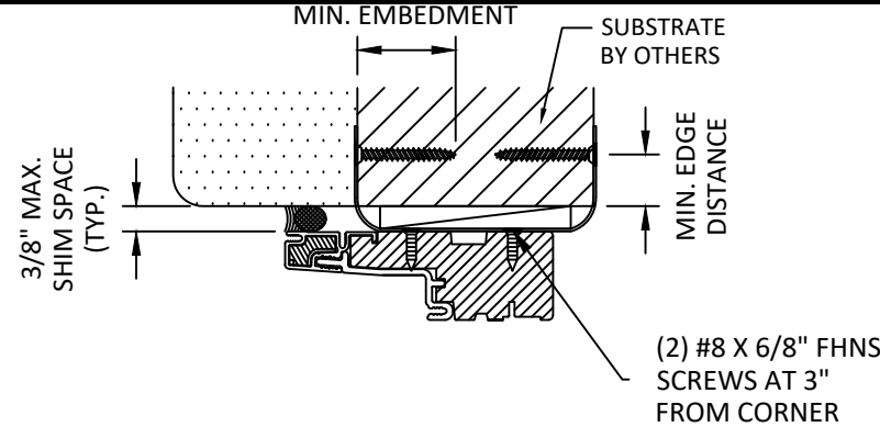
C 10 ANCHOR DETAIL STRAP ANCHOR (WITH 2X BUCK) (SILL & JAMB)
