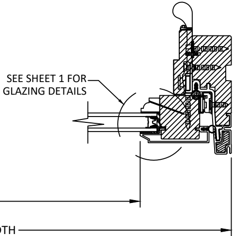
B 8 HORIZONTAL SECTION INSULATED GLASS
