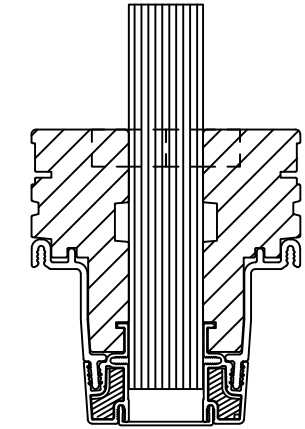
1" X 5 3/16" LVL MULL PROFILE
