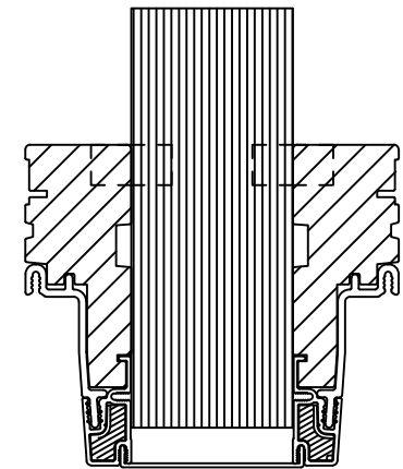
2" X 5 3/16" LVL MULL PROFILE
