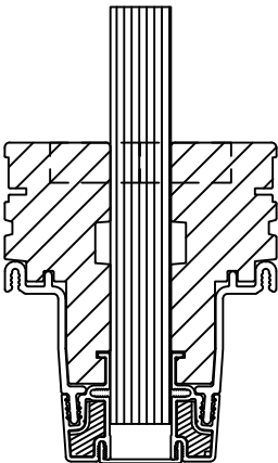
3/4" X 5 3/16" LVL MULL PROFILE
