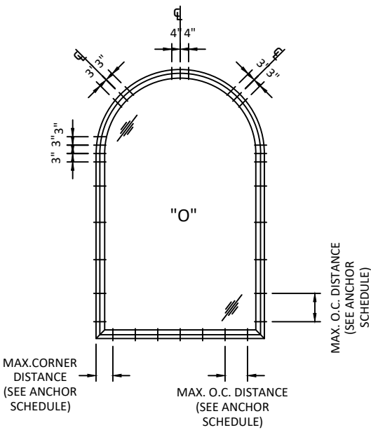
FRAME ANCHORING RADIUS SINGLE UNIT
