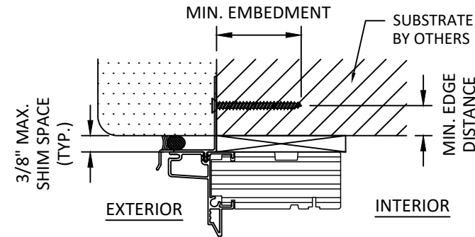
E 10 ANCHOR DETAIL VINYL NAIL FIN W/ DRIP EDGE
