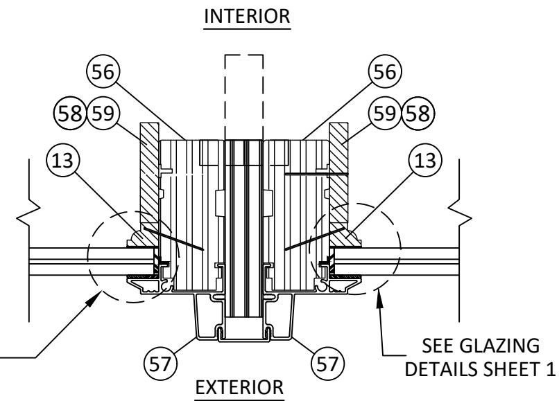
B 9 HORIZONTAL SECTION MONOLITHIC GLASS 3/4" x 3 1/2" MULLION OR 3/4" x 5 3/16"
