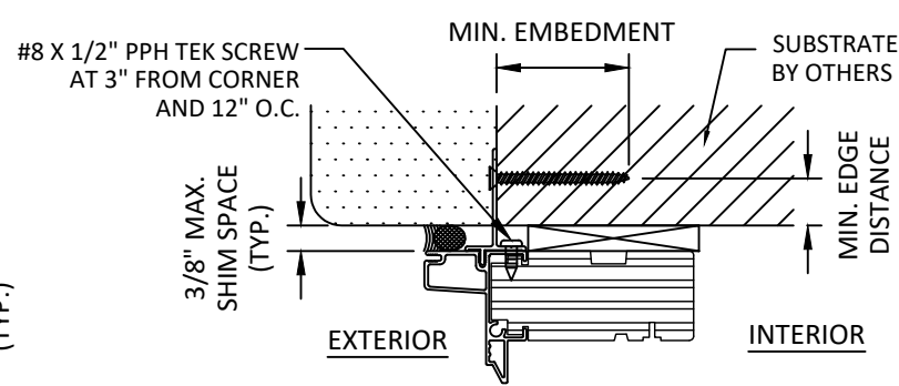
B 10 ANCHOR DETAIL ALUMINUM NAIL FIN
