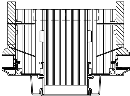
2" X 3 1/2" LVL MULL PROFILE
