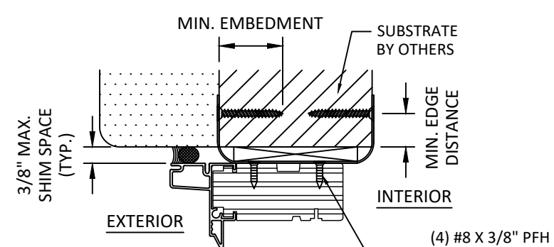
C 10 ANCHOR DETAIL STRAP ANCHOR (WITH 2X BUCK)
