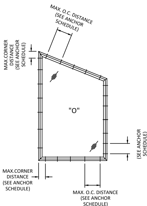
FRAME ANCHORING TRAPEZOID SINGLE UNIT
