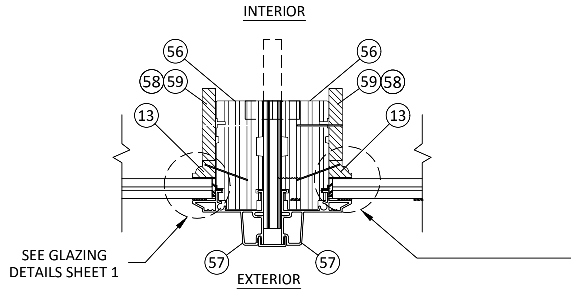
A 9 HORIZONTAL SECTION MONOLITHIC GLASS 1/2" x 3 1/2" MULLION OR 1/2" x 5 3/16"
