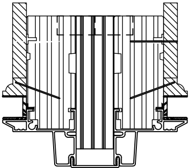
1" X 3 1/2" LVL MULL PROFILE
