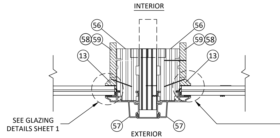
C 9 HORIZONTAL SECTION MONOLITHIC GLASS 1" x 3 1/2" MULLION OR 1" x 5 3/16"
