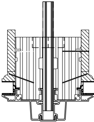
1/2" X 5 3/16" LVL MULL PROFILE
