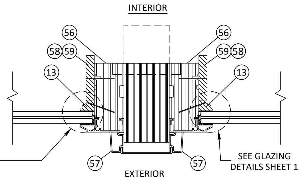
D 9 HORIZONTAL SECTION MONOLITHIC GLASS 2" x 3 1/2" MULLION OR 2" x 5 3/16"
