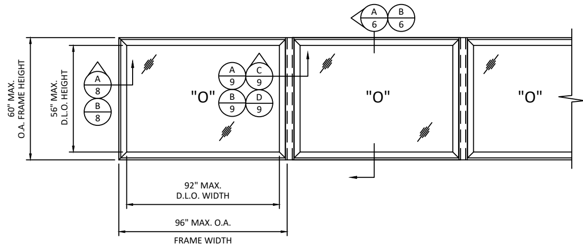
ELEVATION MULLER UNITS HORIZONTAL CONFIGURATION
