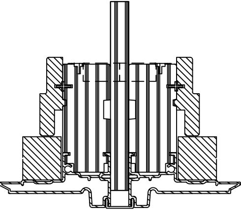
1/2" X 5 3/16" LVL MULL PROFILE
