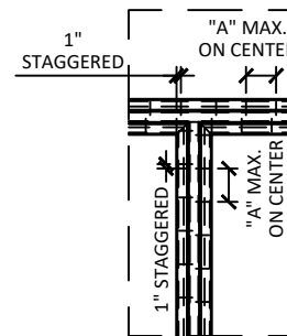
DETAIL 2
