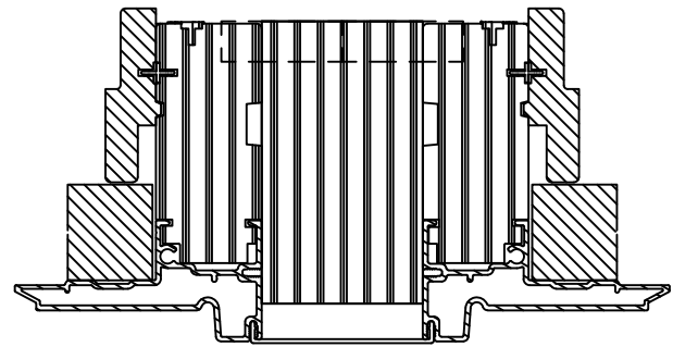
2" X 3 1/2" LVL MULL PROFILE
