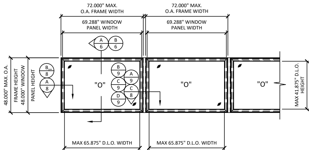
ELEVATION MULLED UNITS (WITH 2\"/>
