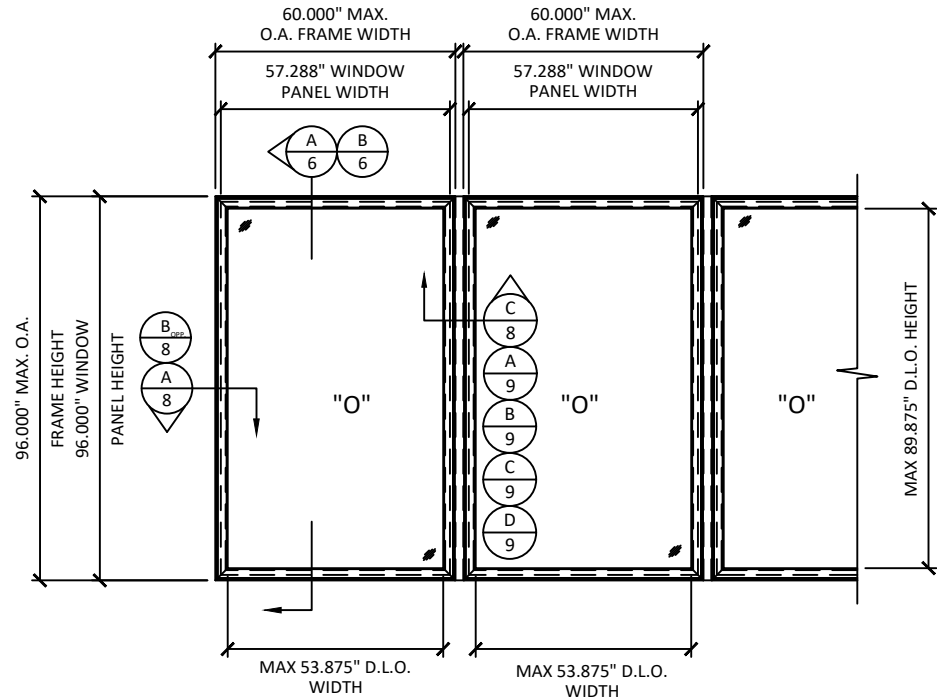
ELEVATION MULLED UNITS (WITH 2\"/>
