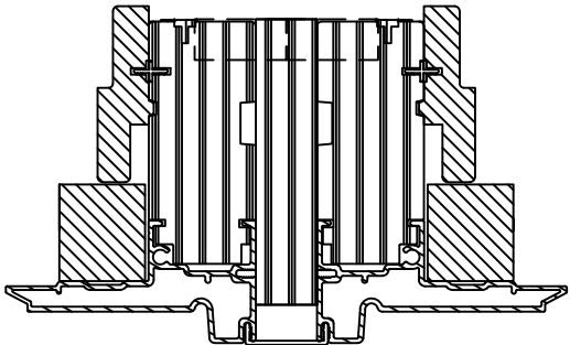
3/4" X 3 1/2" LVL MULL PROFILE
