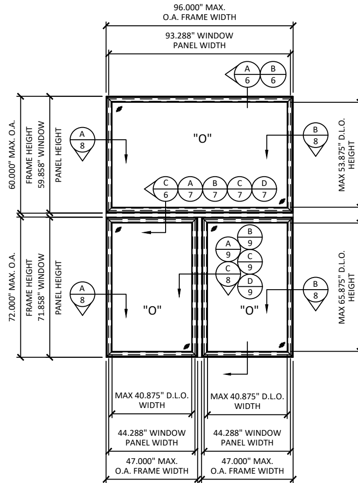
ELEVATION MULLED UNITS (WITH 2\"/>
