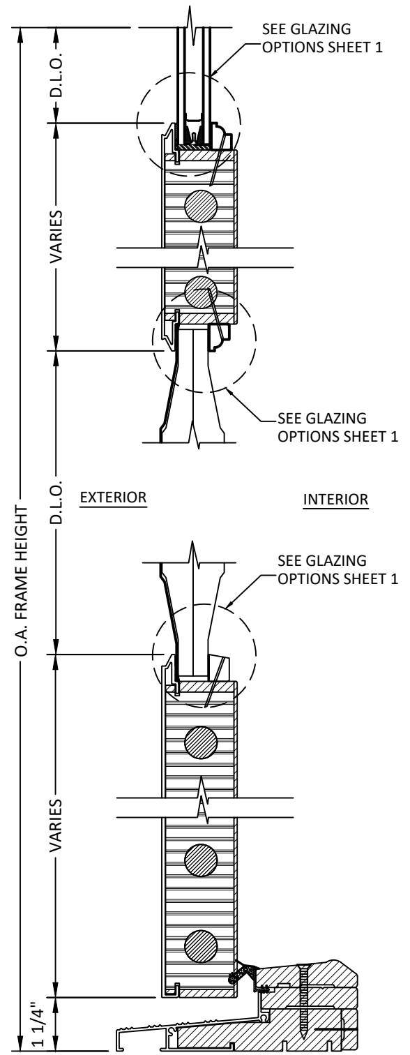
3 3.0 VERTICAL SECTION PANEL WITH MID RAIL
