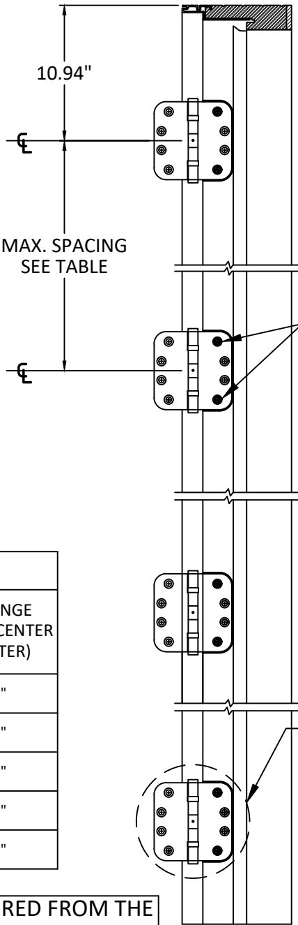
HINGE DETAIL
