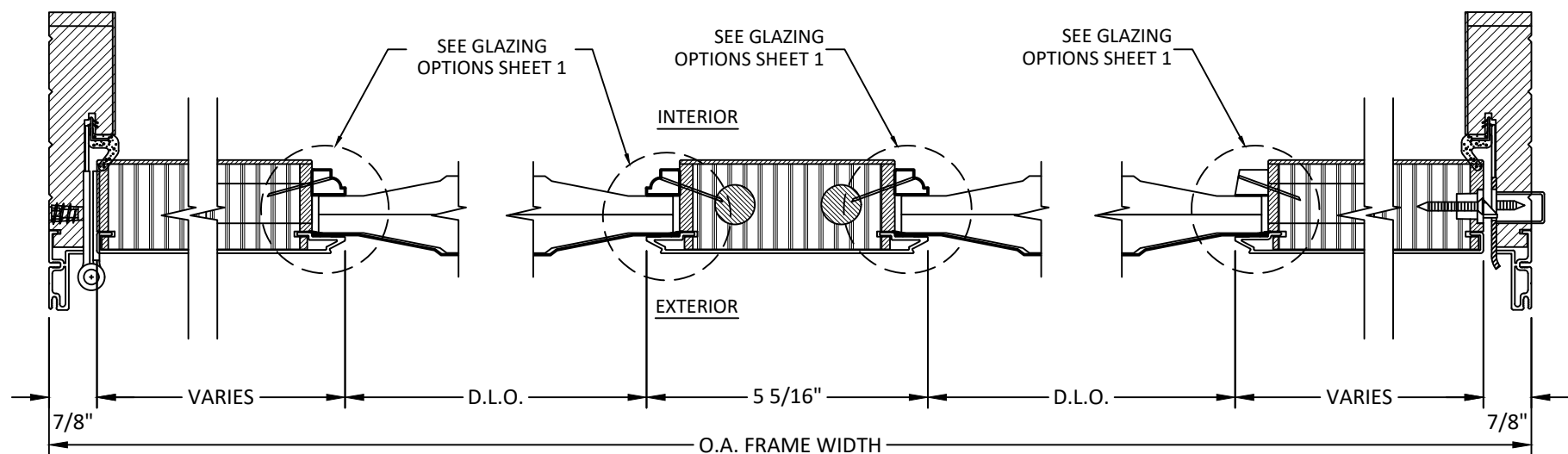
1 4.0 HORIZONTAL SECTION HINGE JAMB WOOD PANEL INSERT
