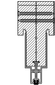
ZERO MULLION
