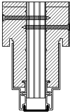
1" X 5 3/16" MULLION
