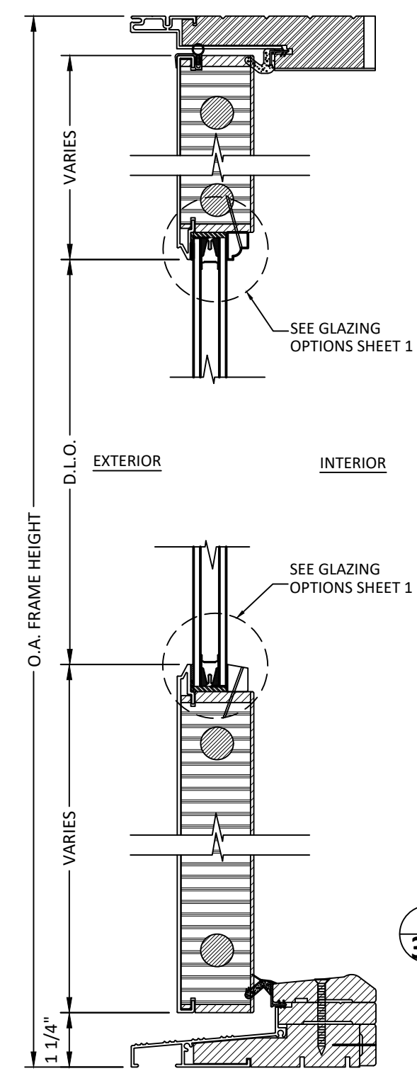
1 3.0 VERTICAL SECTION FULL GLAZED PANEL
