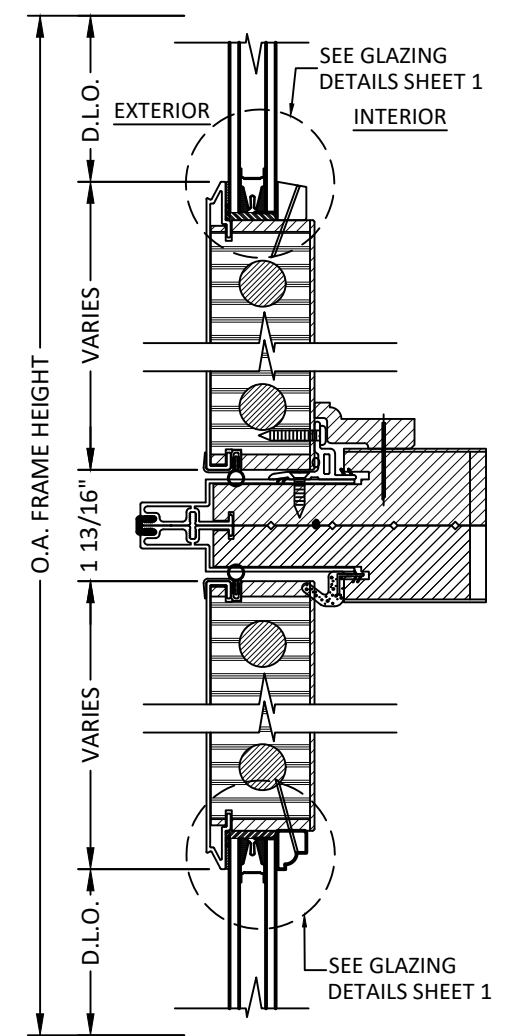
2 3.0 VERTICAL SECTION INSULATED GLASS ZERO MULLION
