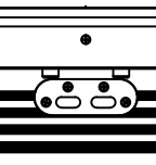
DETAIL D LOOKING DOWN @ SILL (LOCK OPTION 1)
