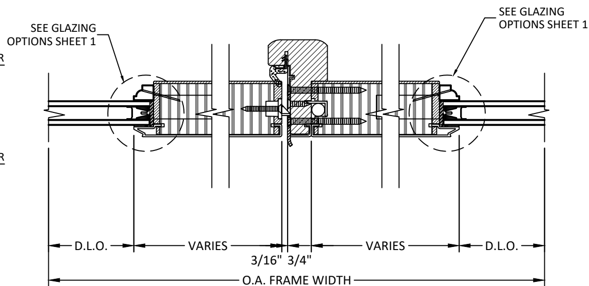
5 4.0 HORIZONTAL SECTION ASTRAGAL
