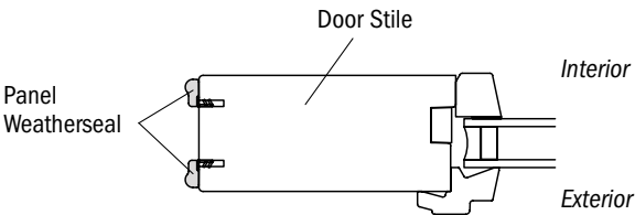
Orientation of Panel Weatherseals on Door Panels (Top View)
