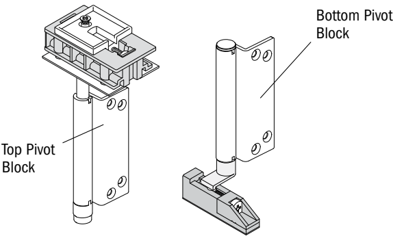
Pivot Set (Right Hand Shown)
