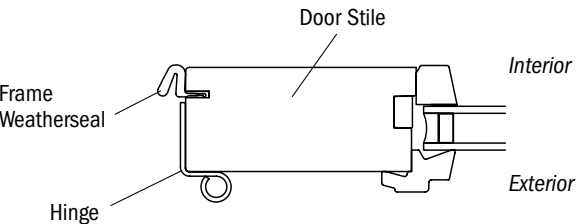
Orientation of Frame Weatherseal on Leading and Jamb Panels (Top View)
