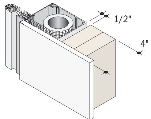
FULL OVERLAP DRYWALL RETURN
