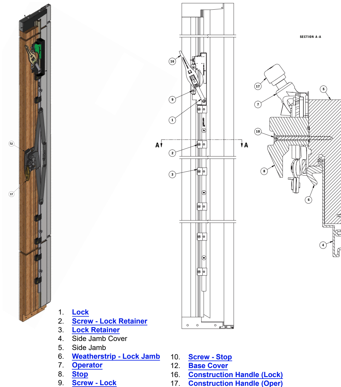
E-Series Hinged Door Lock Jamb Assembly
