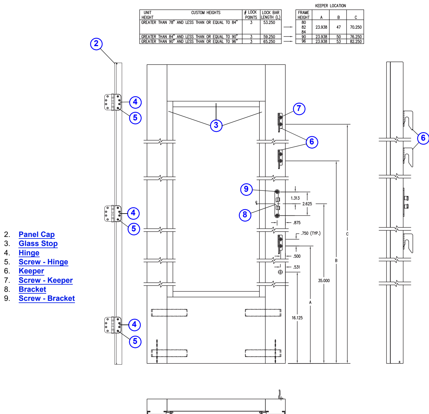
E-Series Venting Hinged Outswing Door Panel
