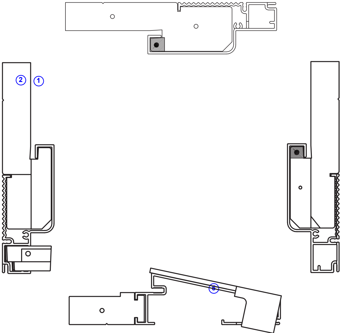
E-Series Hinged Transom Frame Assembly
