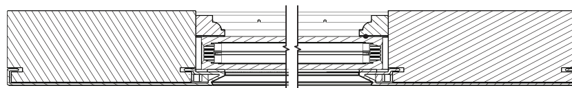
SECTION B-B SHOWN WITH .469 COLONIAL GLASS STOP & DUAL PANE INSULATED GLASS MAXIMUM ALLOWABLE GLASS THICKNESS FOR I.G. UNITS = 27.0 MM OR 1.063"
