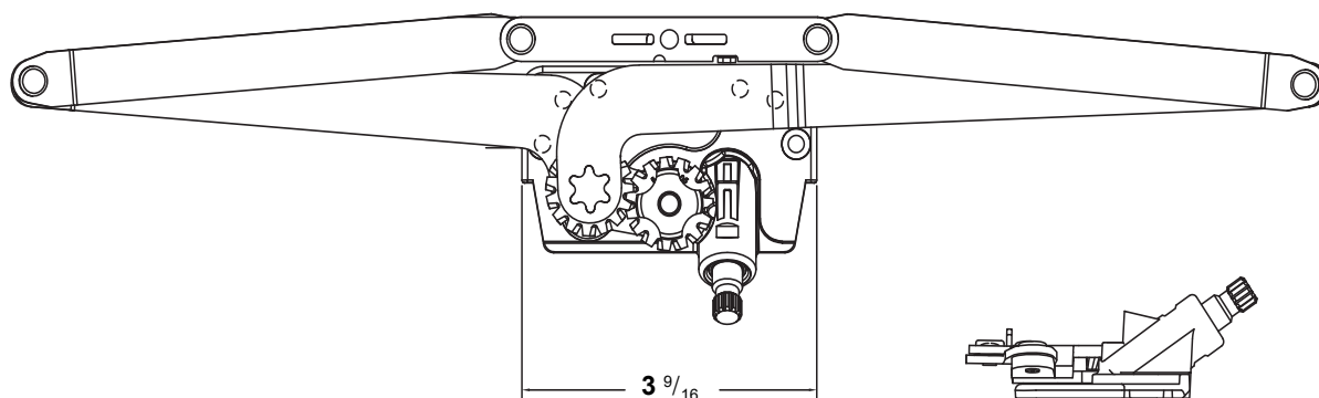
Awning Operator / 16"
