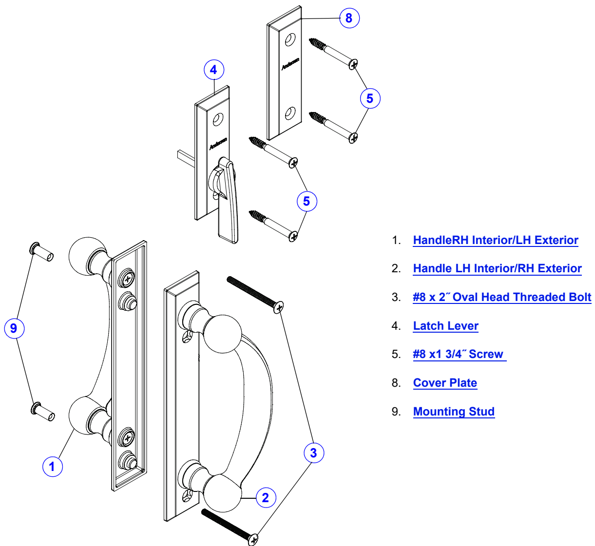
Yuma® Gliding Patio Door Hardware - 2-Panel Trim Set
