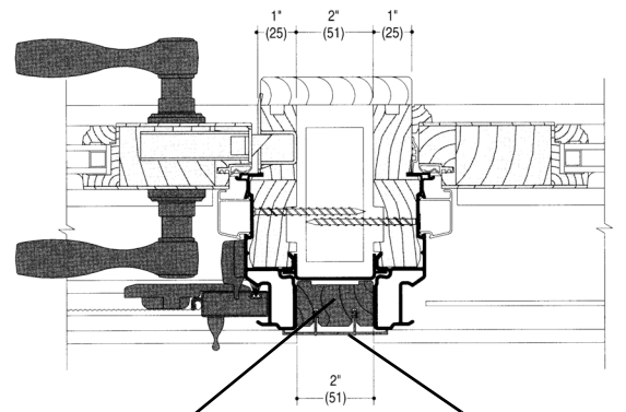
Joining Strip Exterior Trim Strip Hinged Door Support Mullion
