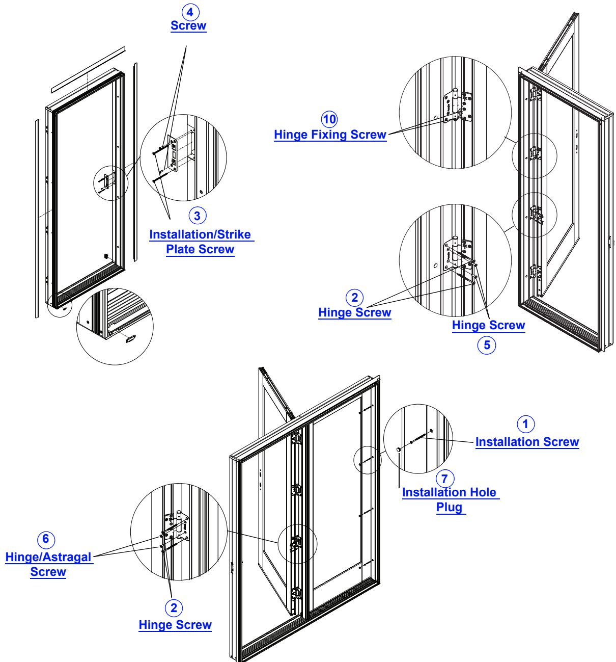
200 Series Hinged Doors - Screw Usage
