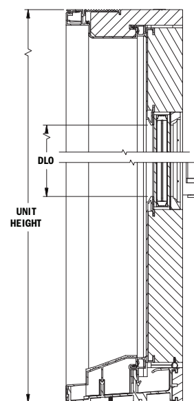
SECTION B-B
