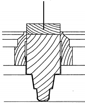
Factory Mullion Interior Casing 2" Face
