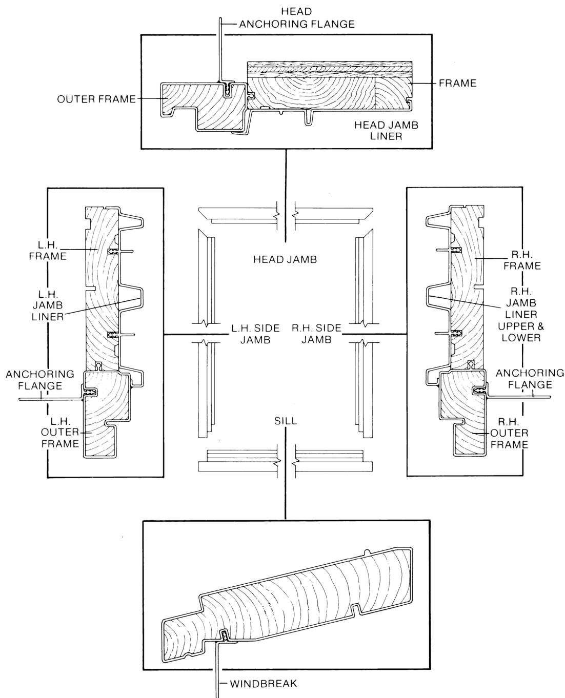
Perma-Shield® Narroline® Frame Assembly
