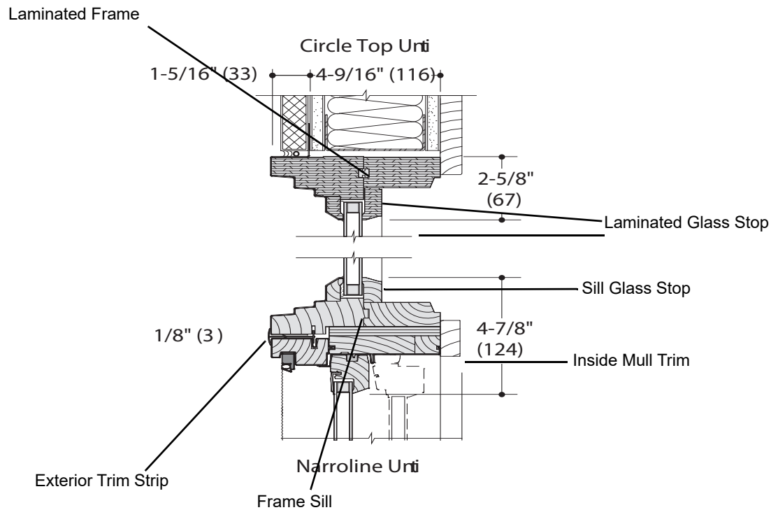
Double-Hung Circle Top™ Transom Joining
