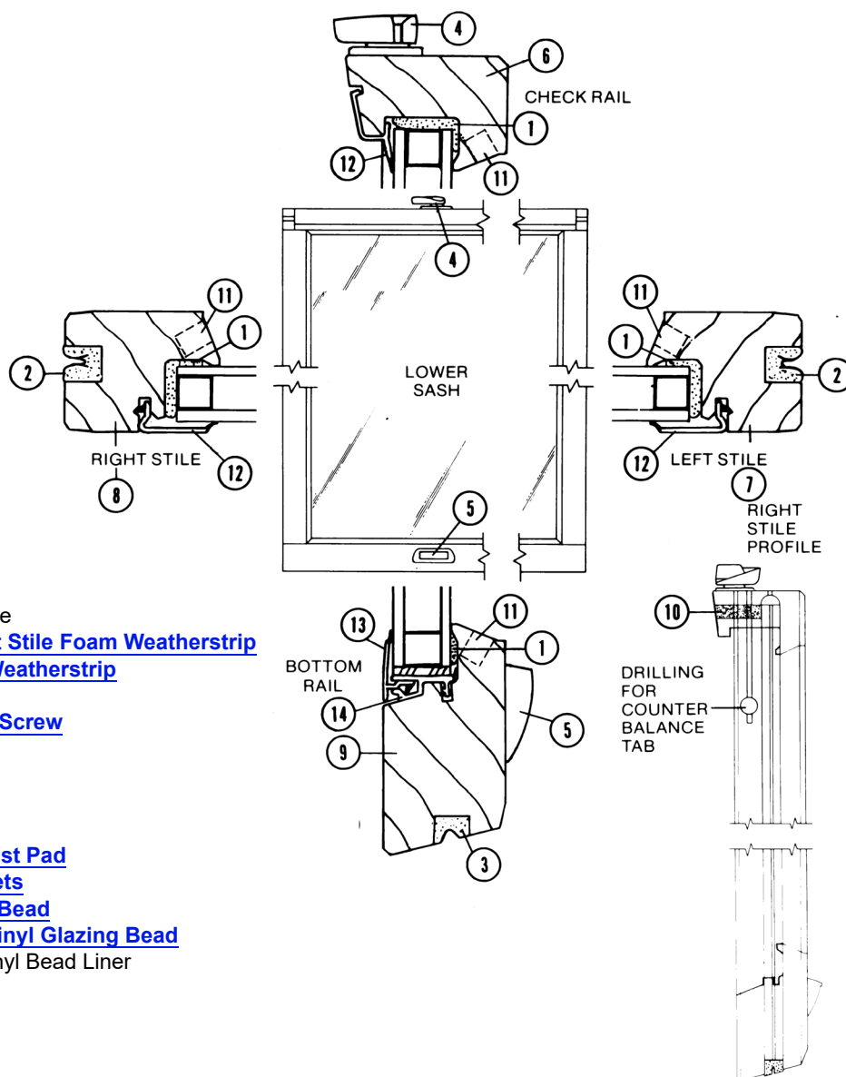
Perma-Shield® Narroline® Lower Sash Parts - Low E and Dual Pane 5/8"
