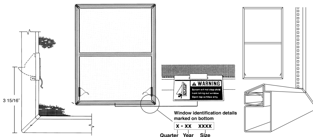
Perma-Shield® Narroline® Full Window Insect Screen
