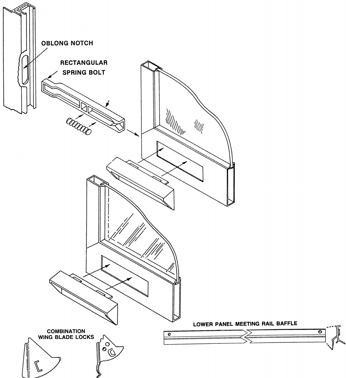
Perma-Shield® Narroline® Combination Unit Panel - Lower / Square Bolt
