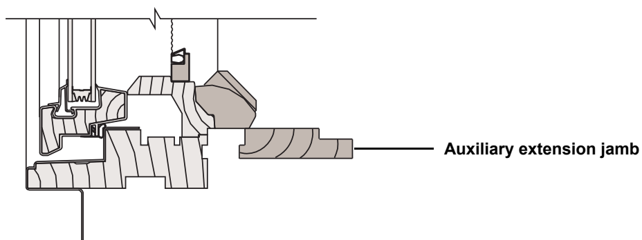
Perma-Shield® Enhanced Casement Auxiliary Extension Jambs
