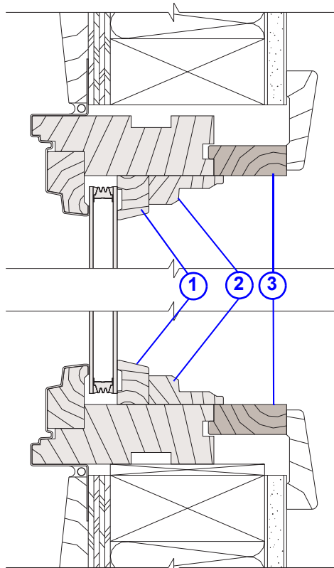
Vertical Section
