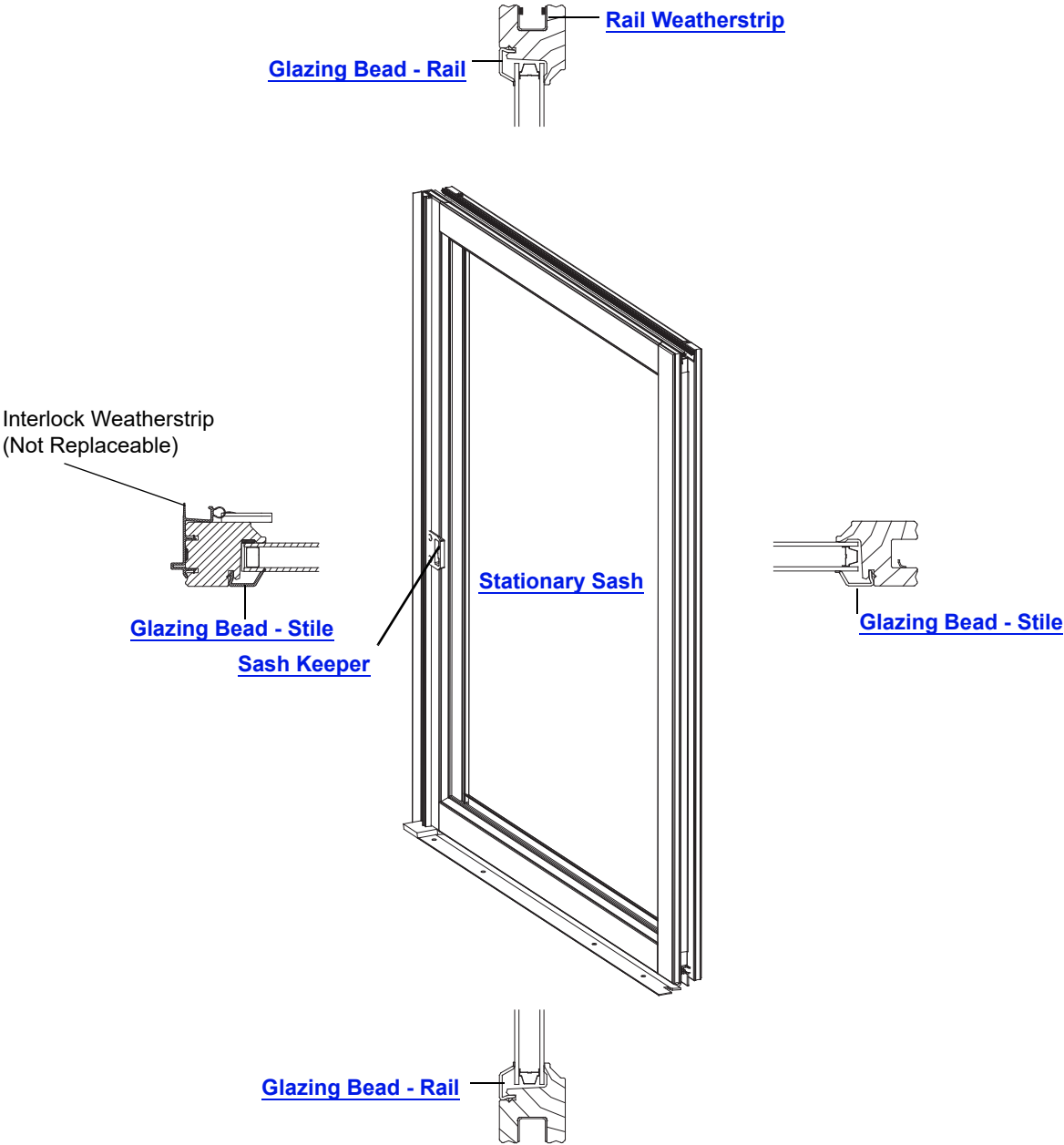
200 Series Gliding Window Stationary Sash
