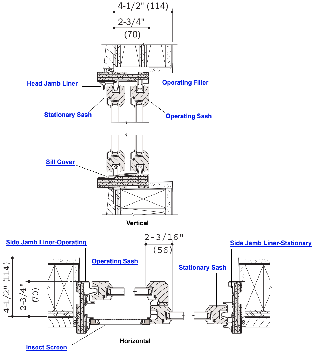
200 Series Gliding Window Frame Assembly
