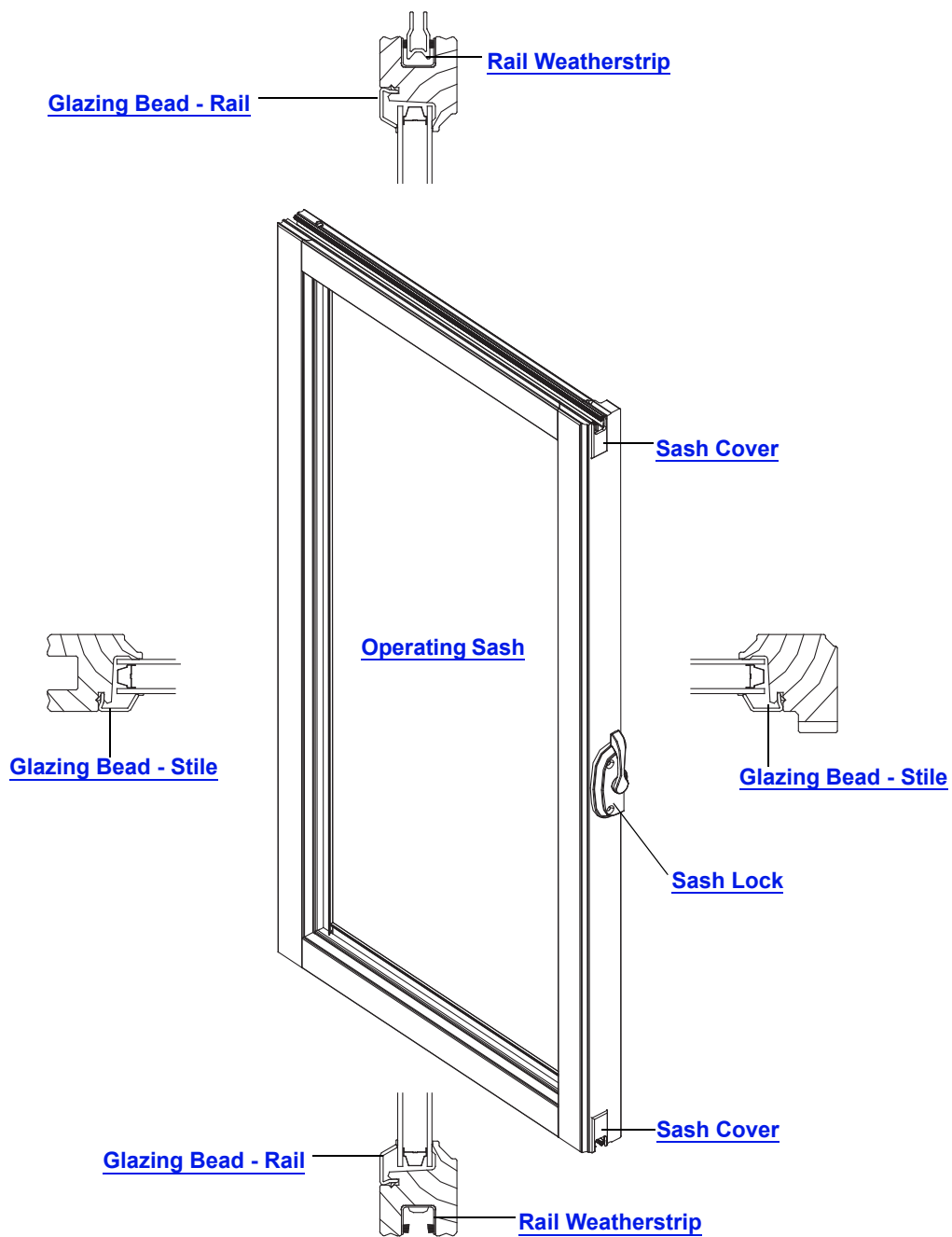
200 Series Gliding Window Operating Sash
