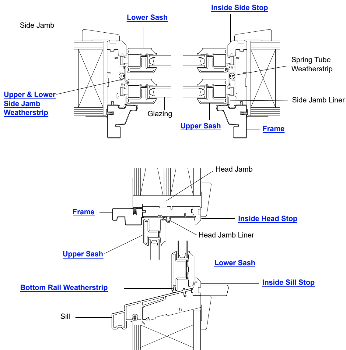
Woodwright® Double-Hung Frame Assembly
