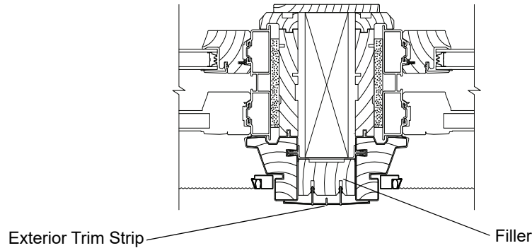
Woodwright® Double-Hung Support Mullion
