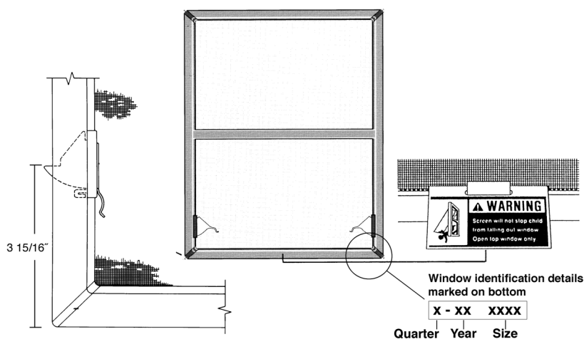
Woodwright® Double-Hung Full Insect Screen
