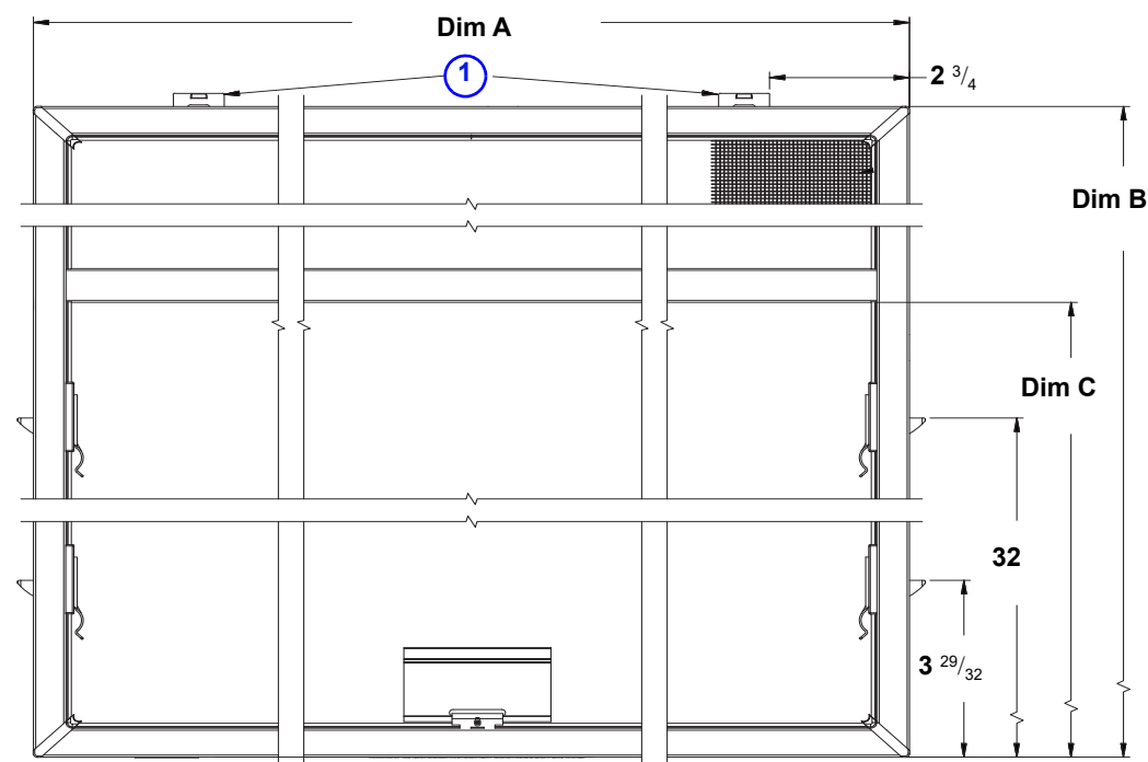
Woodwright® Insert Window Full Insect Screen
