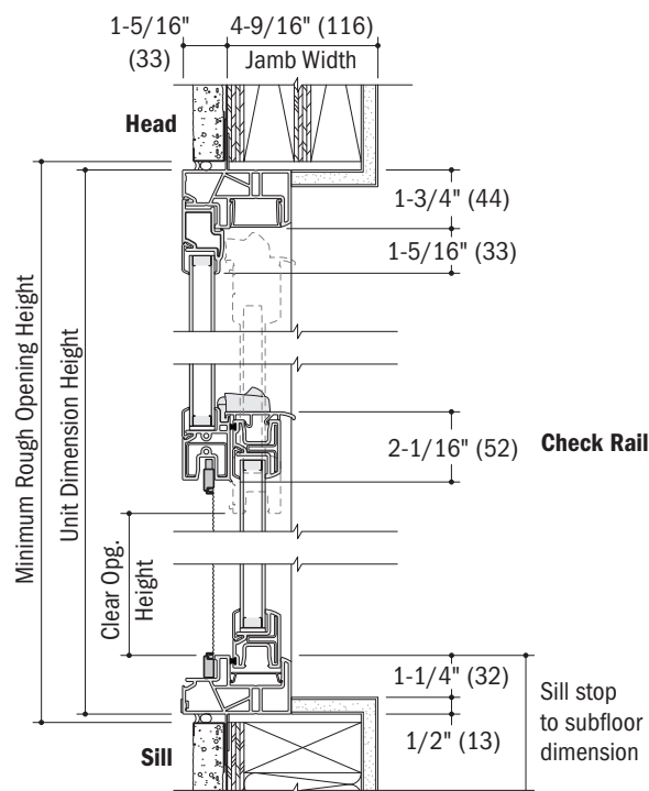
Vertical Section Single-Hung Window
