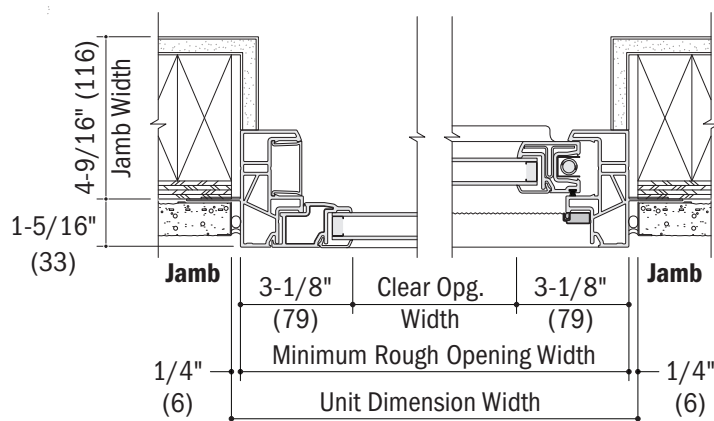
Horizontal Section Single-Hung Window
