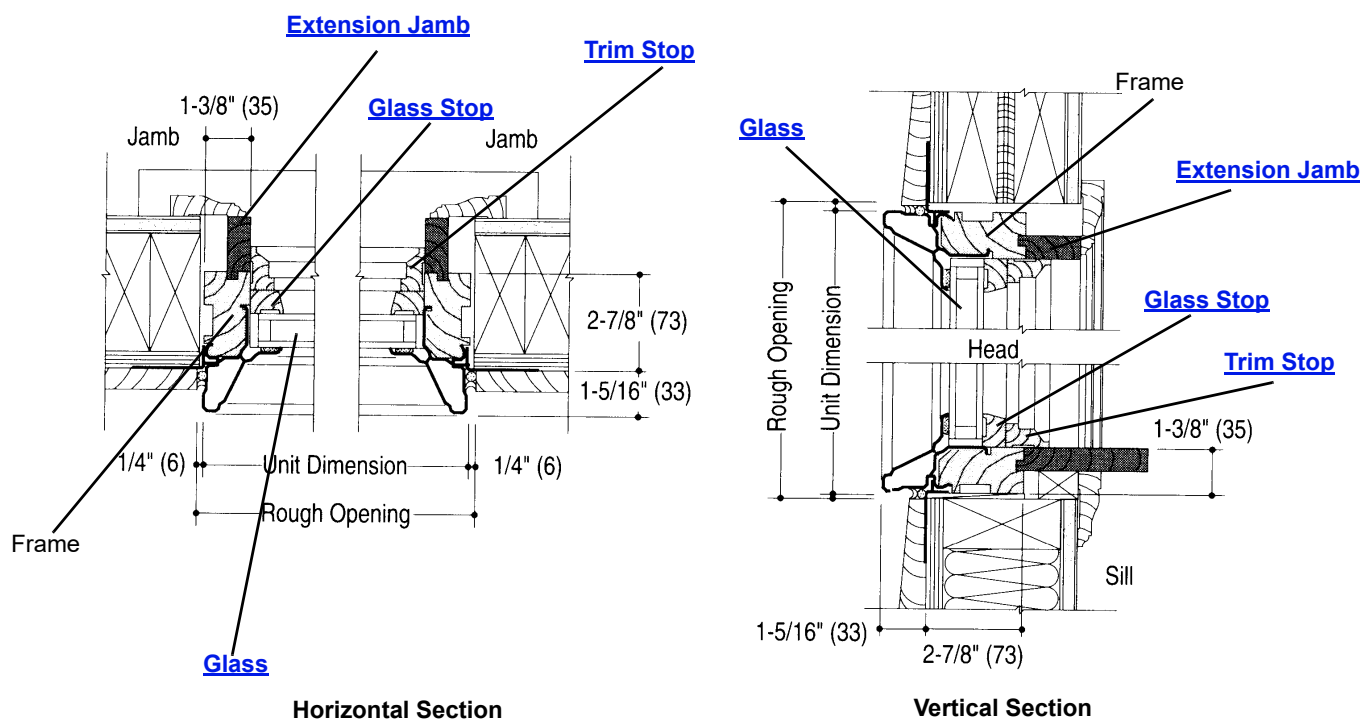
Flexiframe Frame Assembly
