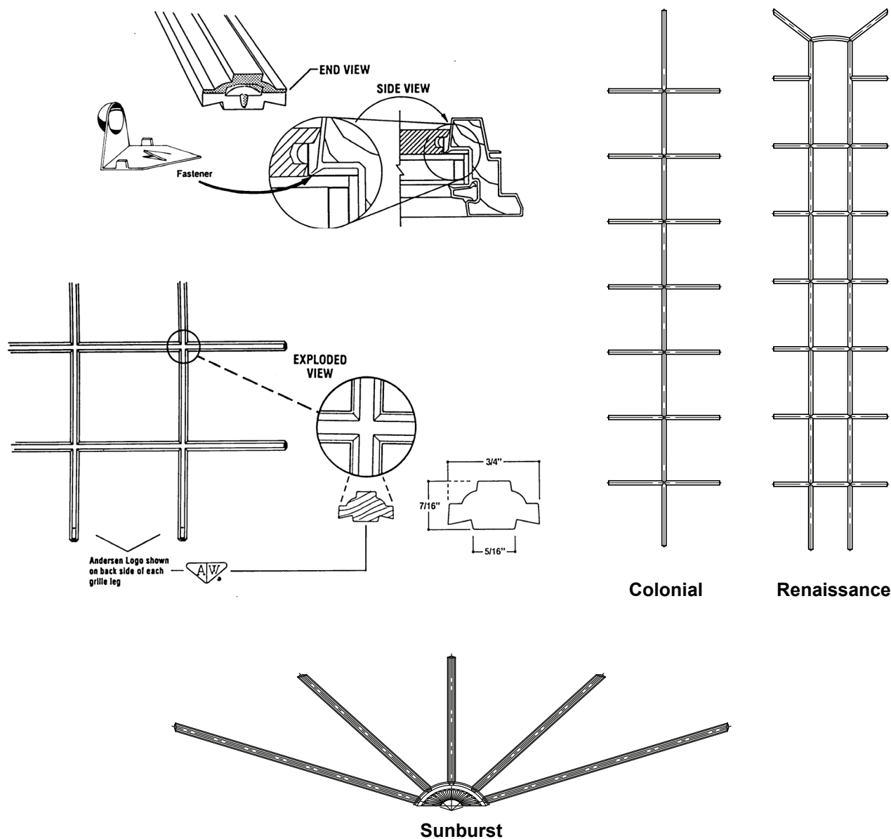
Arch Window Wide Profile Interior Grilles
