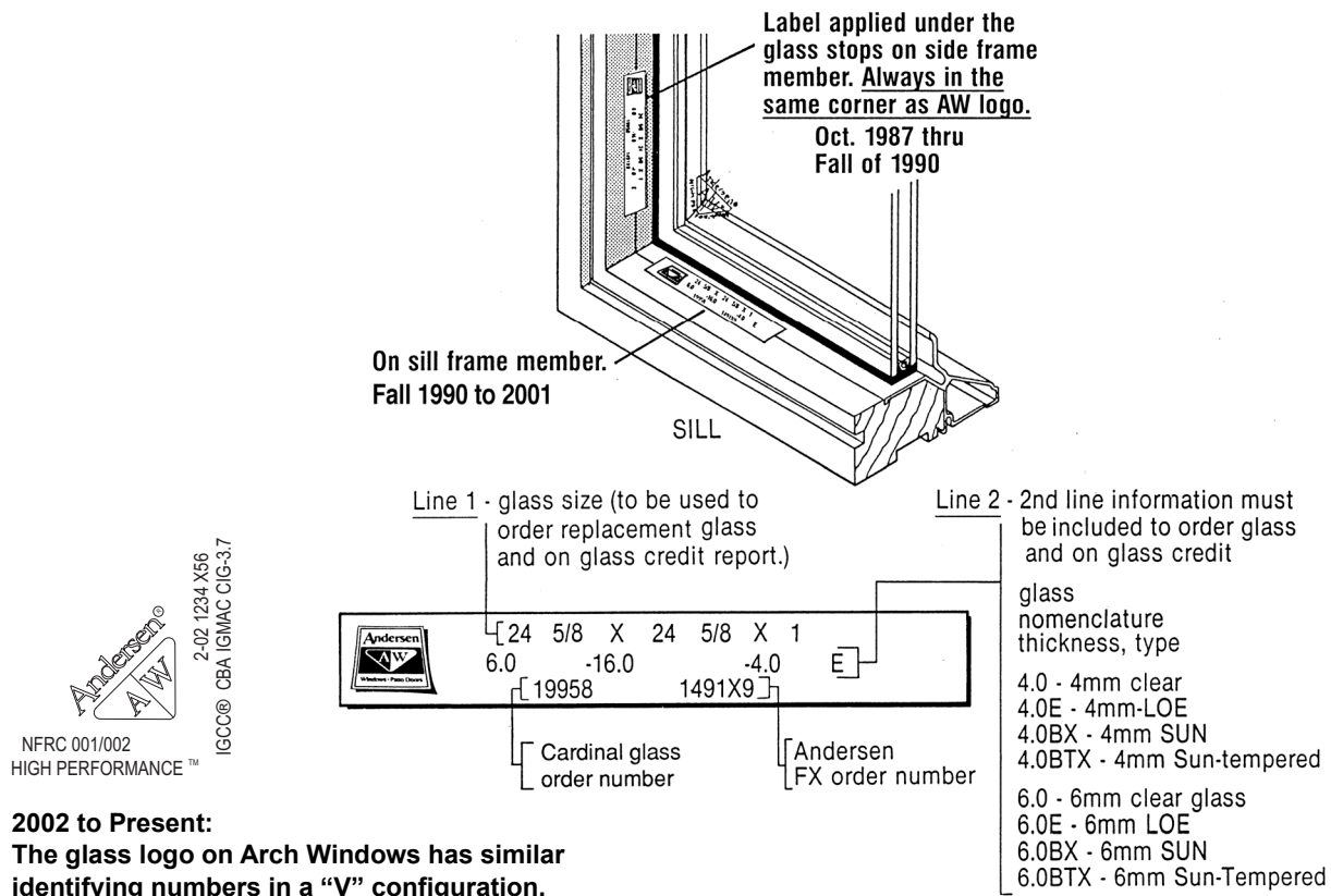
Arch Glass Dimension Label
