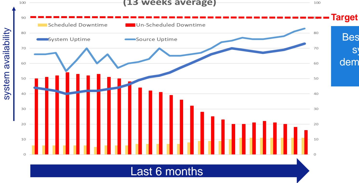
NXE:3400B Availability Performance - last 6 months (13 weeks average)
