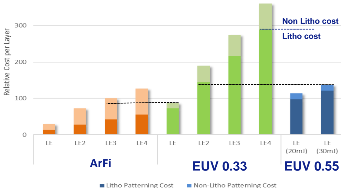
Total patterning cost comparison: ArFi, EUV 0.33, EUV 0.55
