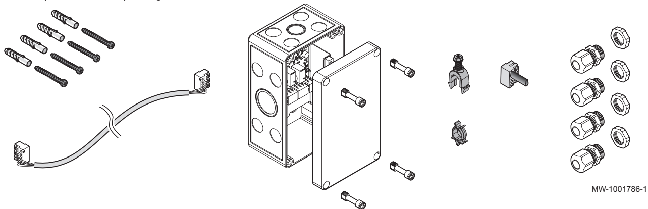
Fig.9 Composition of the package
