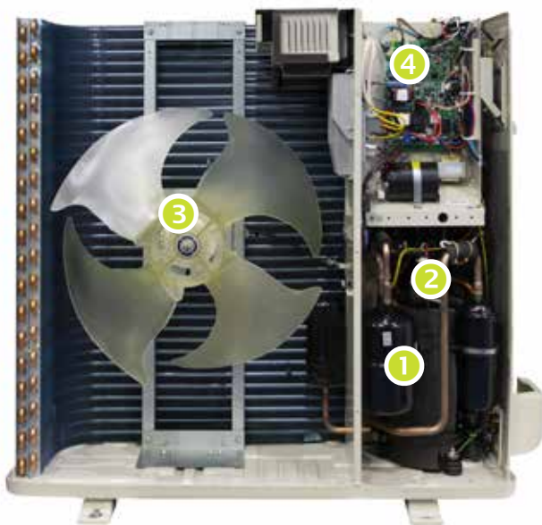
Modello HPS 6/8
