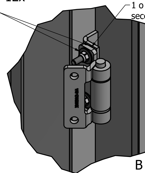
(15) 4VMC00000168 RONDELLA D:7 MM ZINCATA 12x
