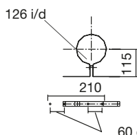
Wall bracket Part No. MG410087863
