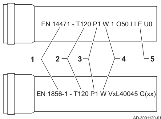
Fig.11 Sample string
