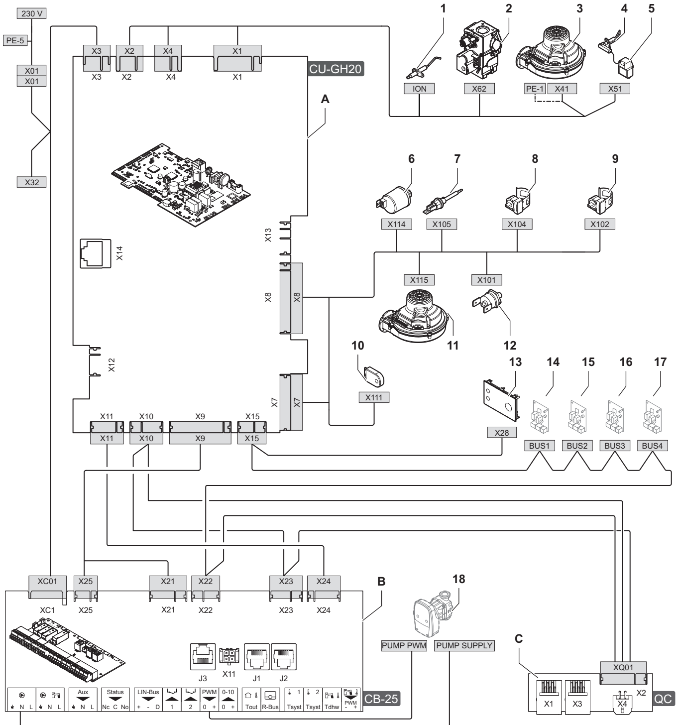
Fig.7 Electrical diagram for boiler types 50 - 60 - 70
