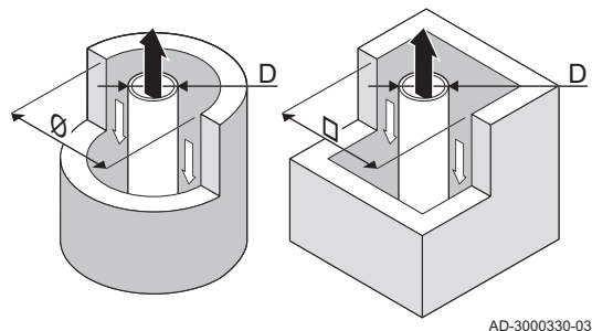
Fig.10 Minimum dimensions of shaft or duct C 93
