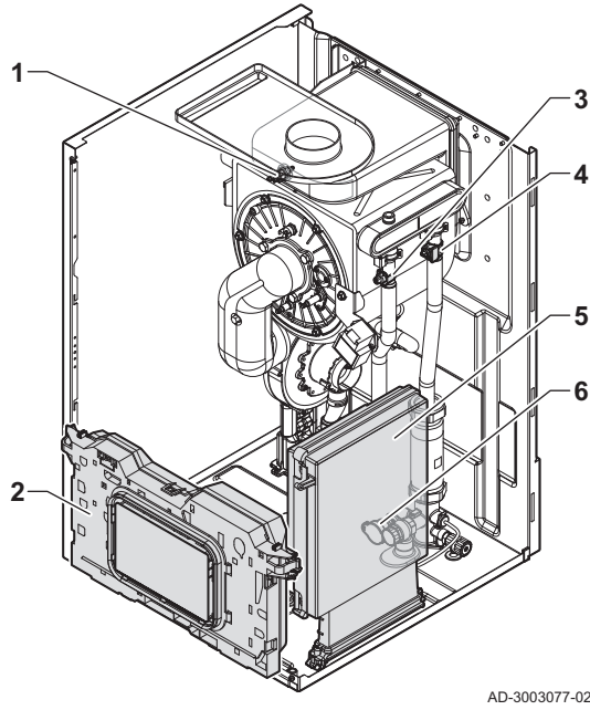
Fig.4 Sensors and boxes
