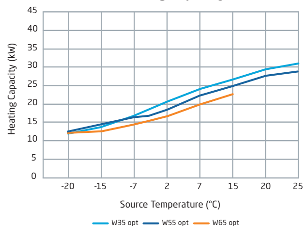
Heating Capacity
