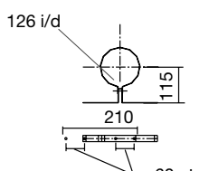
Wall bracket Part No. MG410087863
