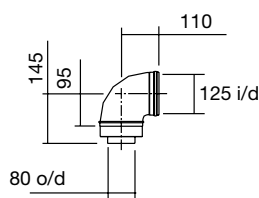
90° Bend Part No. MG410084460 90° Boiler short bend Part No. MG410084810
