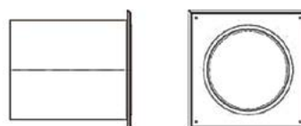
Cover plate 300mm x 300mm with sleeve 250mm x 300mm Part No. MG410081362
