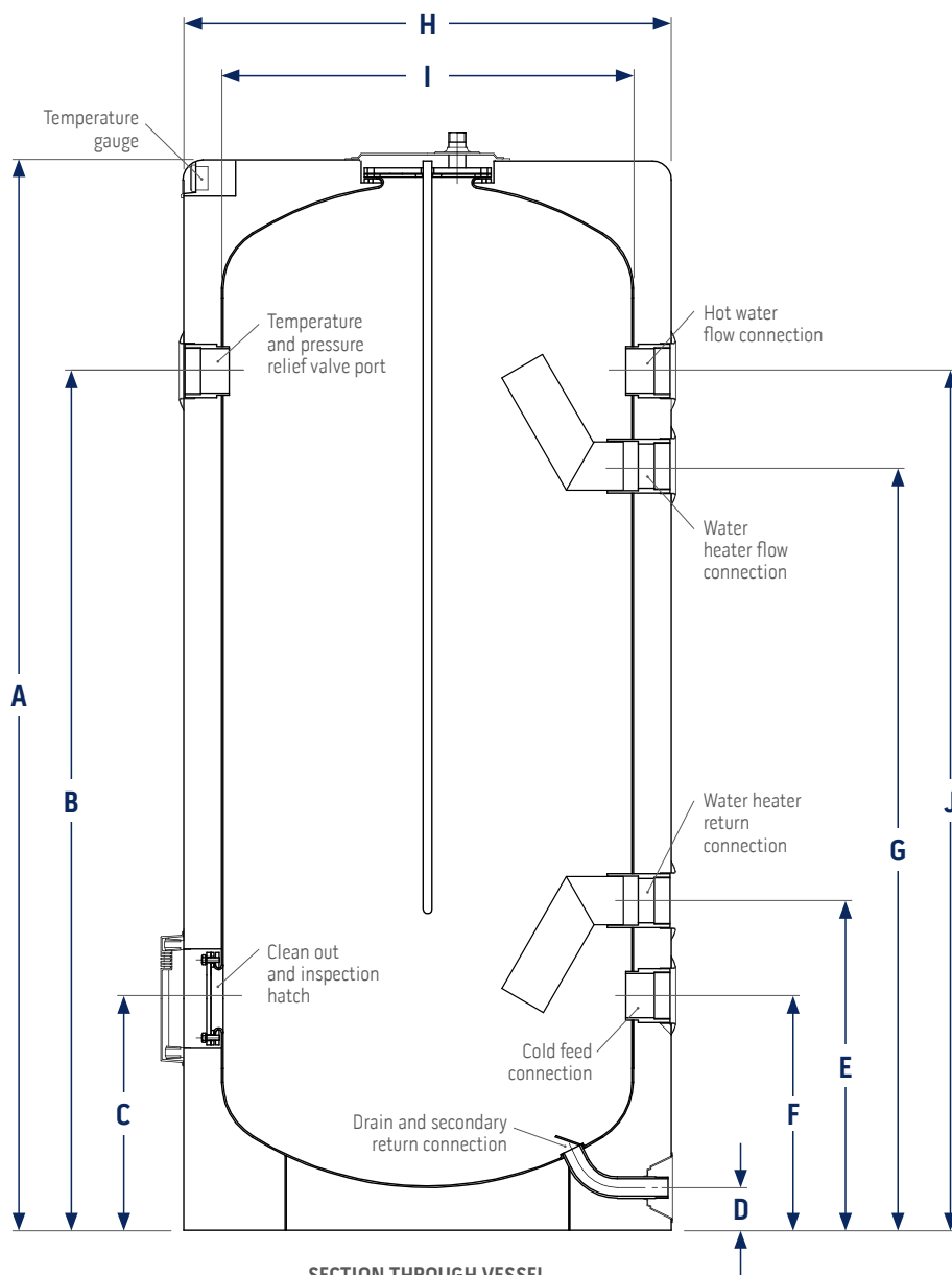
SECTION THROUGH VESSEL
