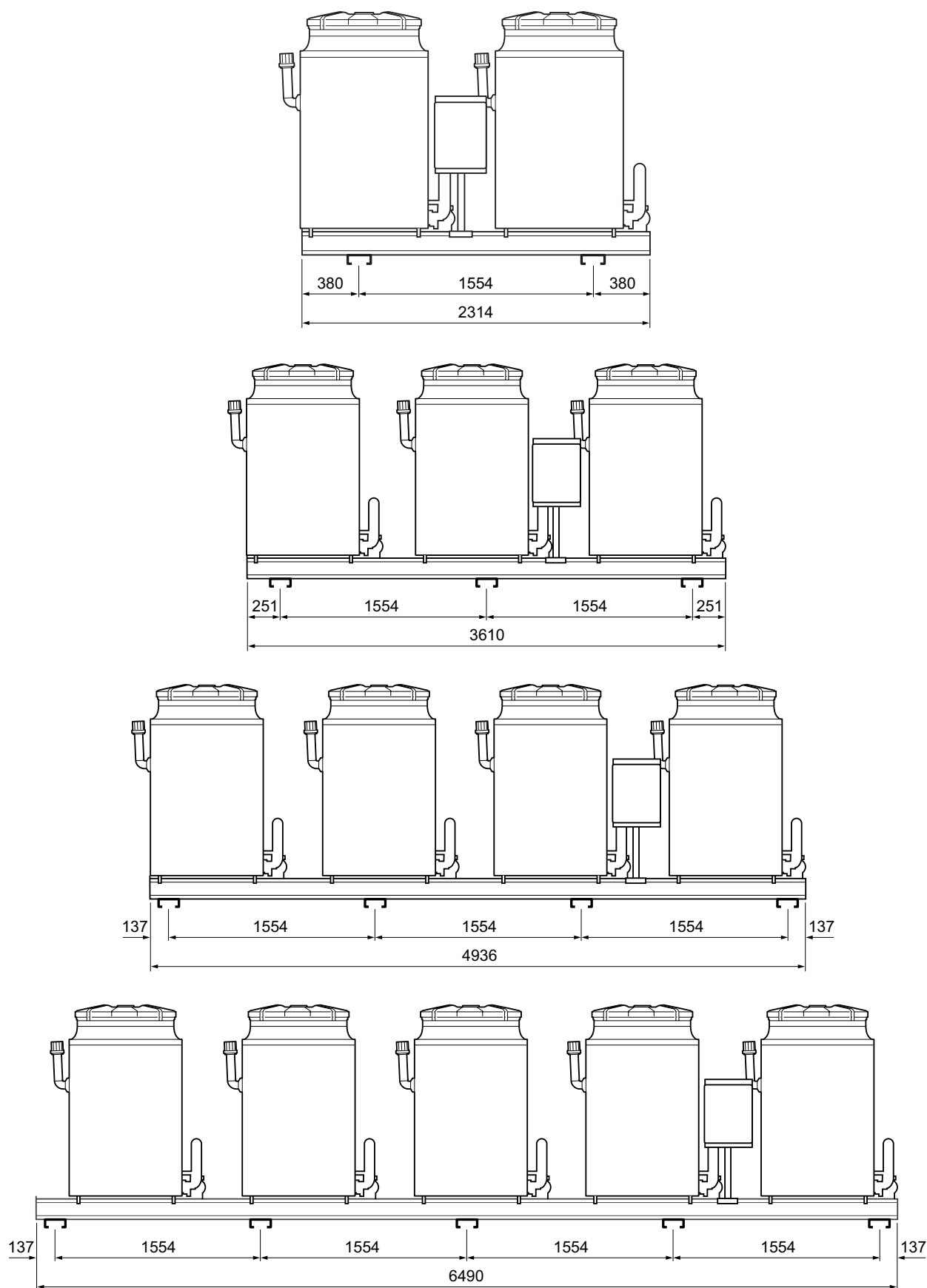
Skids cascadeframes
