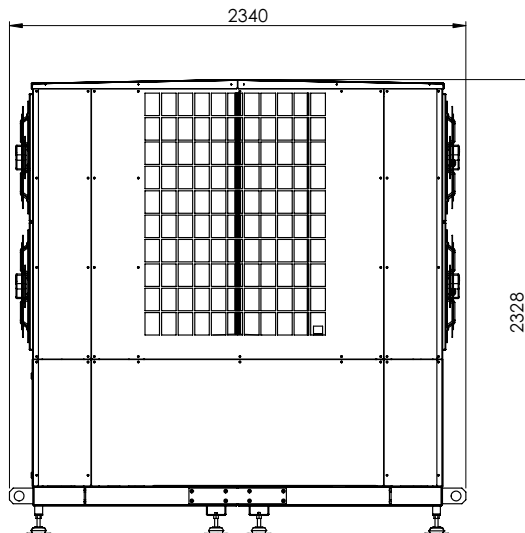
Remeha E-HP AW 172/176
