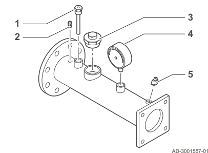
Fig. 6 Flow pipe
