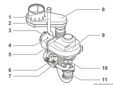
Fig. 4 - Gas – Air unit
