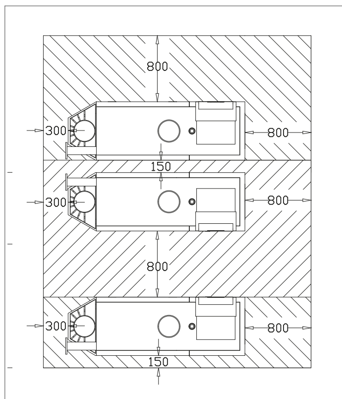
Multiple configuration
