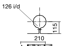
Wall bracket Part No. MG410087863
