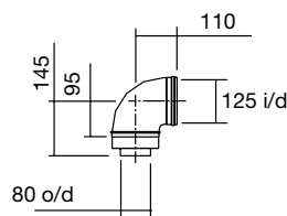
90° Boiler short bend Part No. MG410084810 90° Bend Part No. MG410084460
