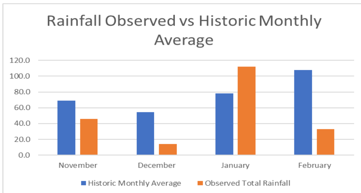
Figure 5-1 Rainfall received compared to historic monthly averages (Source BOM & M12 West AWS)
