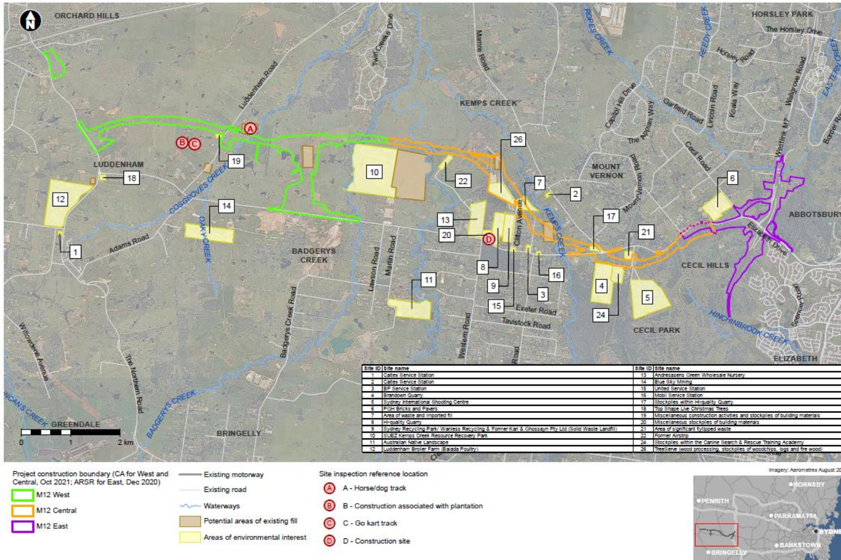
Figure 4-1 Areas of Environmental Interest (West package – Green section)
