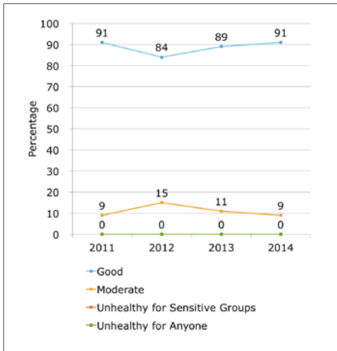
Figure 1 | Percent of Days by Each Air Quality Rating, City of Charlottesville, 2011–2014. Source: Environmental Protection Agency, 2016.
