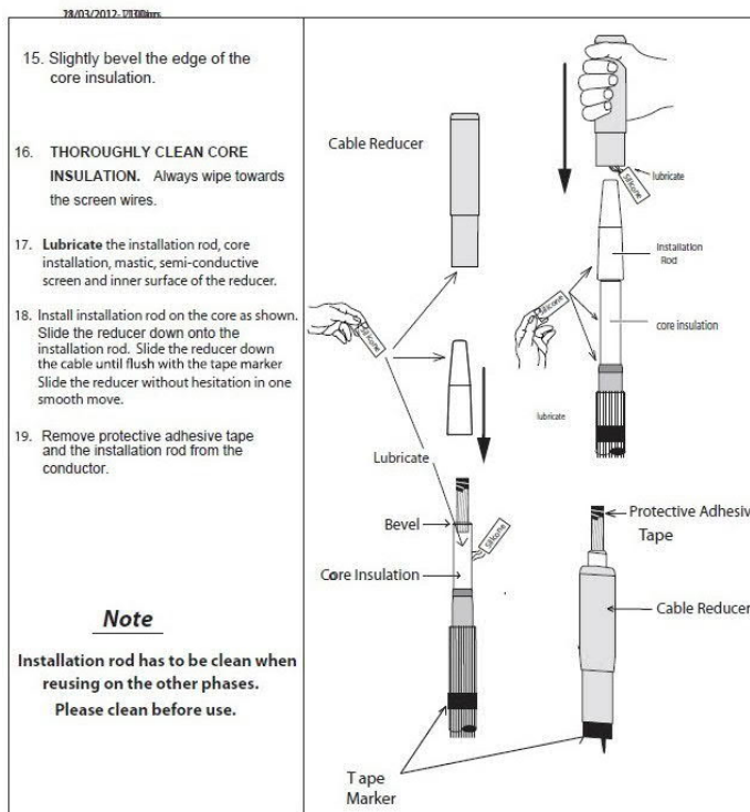
Figure 3 above right: The use of the lubricated installation rod enables the cable reducer to be installed correctly onto the core
