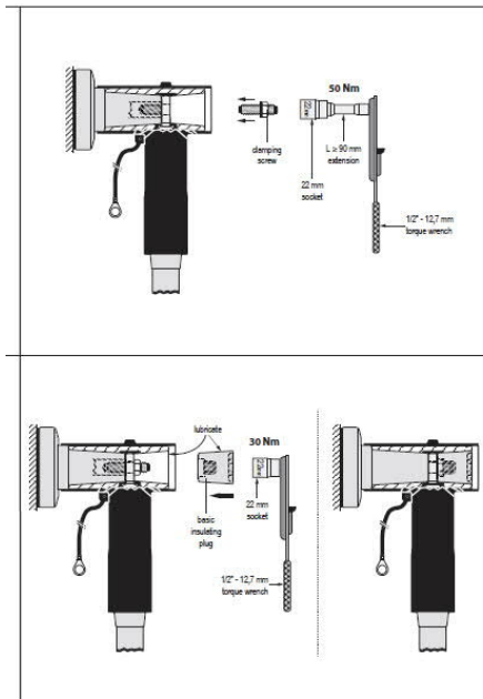
Figure 1 at left: (Previous connection method) the locking bolt is inserted through the palm of the lug after the elbow is positioned on the bushing. The insulating plug is then secured in place.
