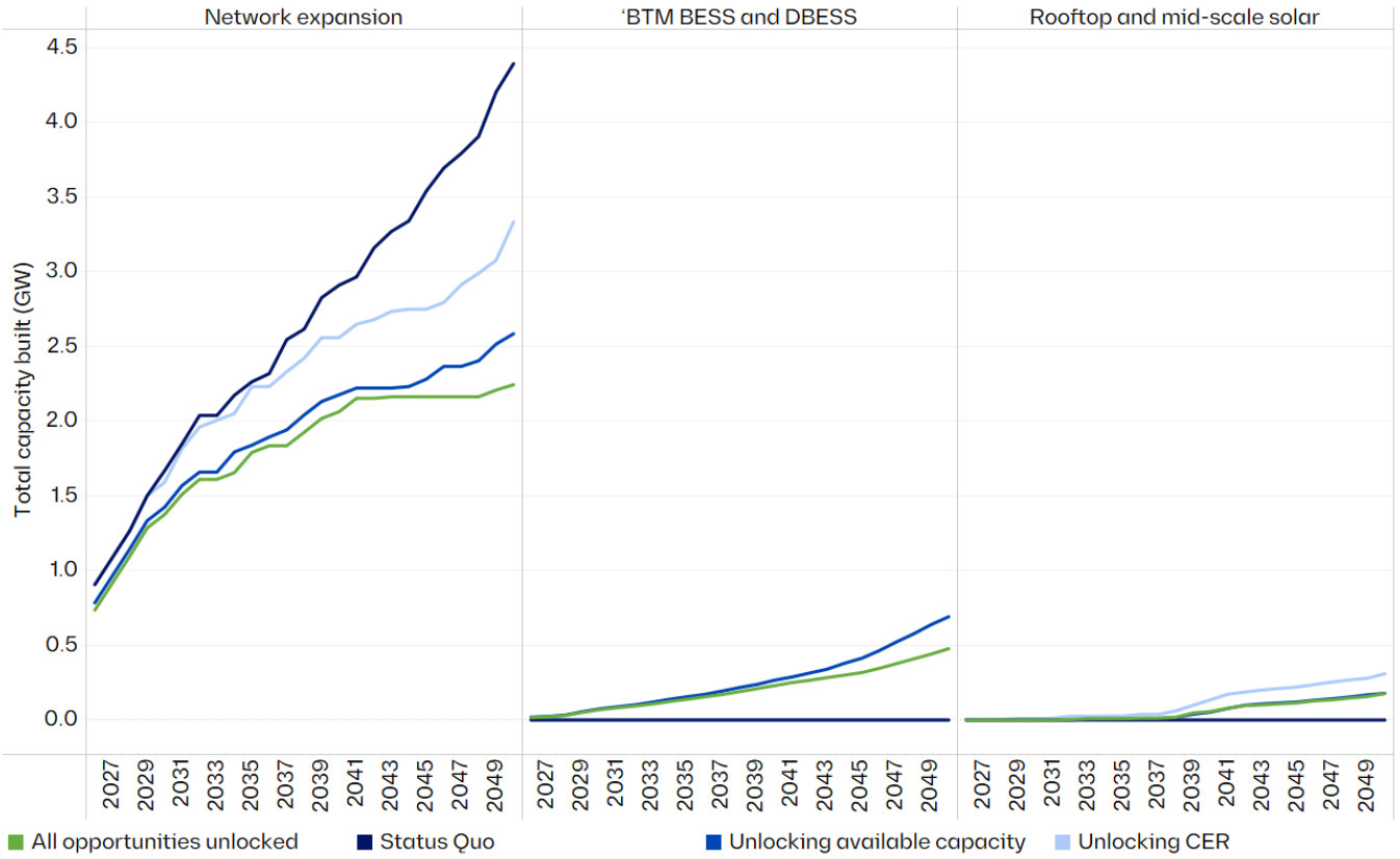
Figure D7: NSW-wide investment outcome in Status quo, Unlocking available capacity, Unlocking CER and All opportunities unlocked
