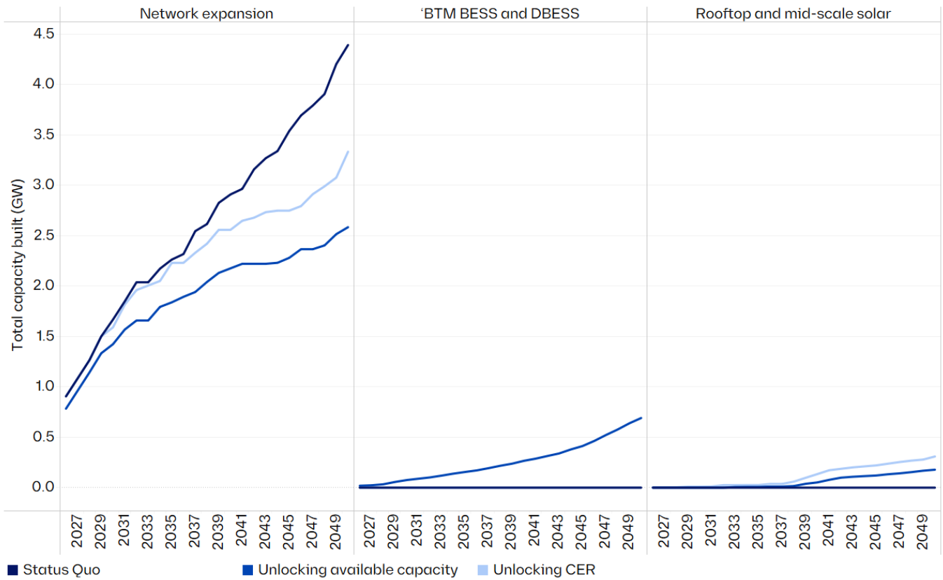
Figure D6: NSW-wide investment outcome in Status quo, Unlocking available capacity and Unlocking CER – Customer transformation and Optimistic case
