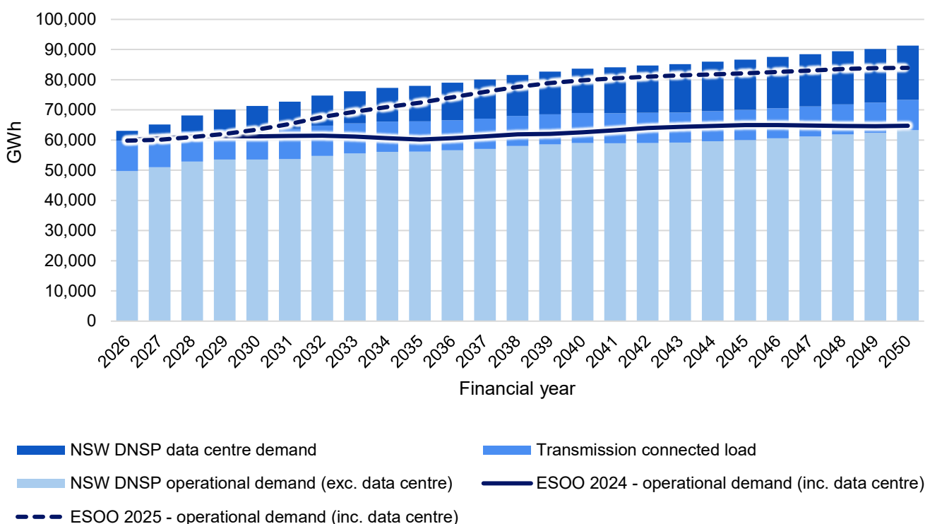
Figure B9: NSW operational demand (excluding hydrogen) – Falling short
